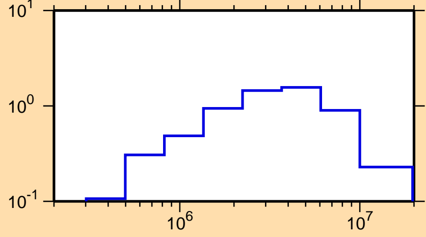
\sigma vs. E for ^{63}\text{Fe}(n,\text{inel.})
