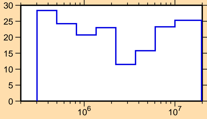
\Delta\sigma/\sigma vs. E for ^{63}\text{Fe}(n,\text{el.})
