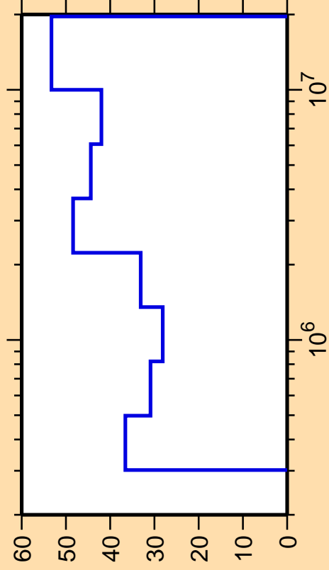
\Delta\sigma/\sigma vs. E for ^{63}\text{Fe}(n,n_1)
