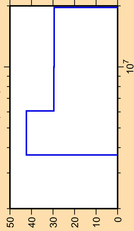
\Delta\sigma/\sigma vs. E for ^{63}\text{Fe}(n,2n)
