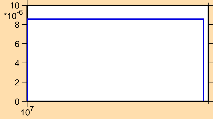
\sigma vs. E for ^{63}\text{Fe}(n,d)
