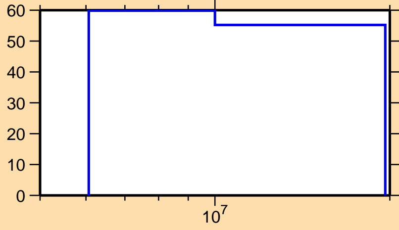
\Delta\sigma/\sigma vs. E for ^{63}\text{Fe}(n,ncont.)
