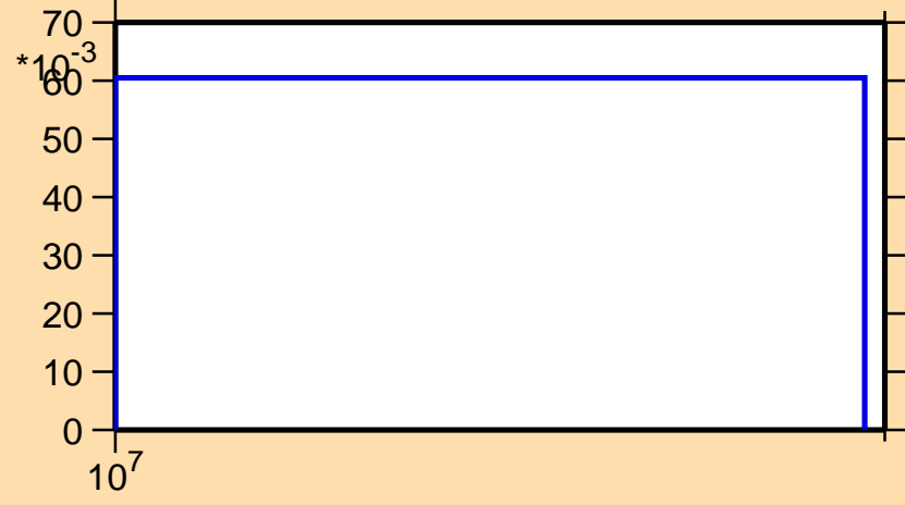
\sigma vs. E for ^{63}\text{Fe}(n,3n)
