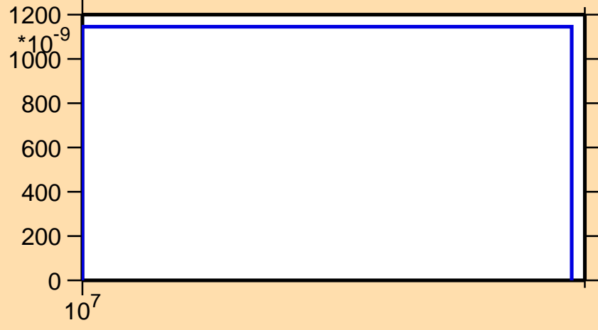
\sigma vs. E for ^{63}\text{Fe}(n,\alpha)
