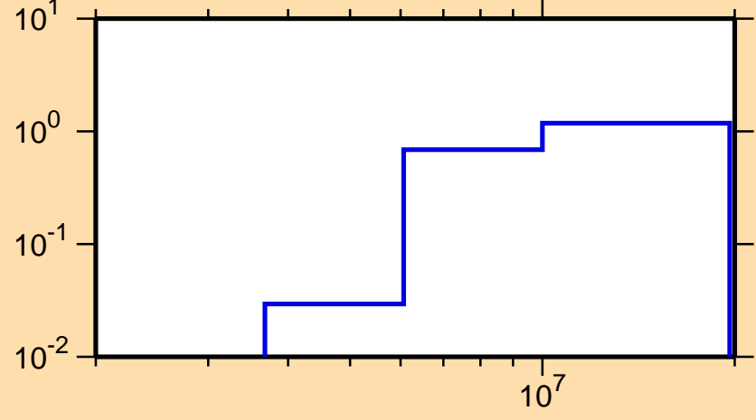
\sigma vs. E for ^{63}\text{Fe}(n,2n)
