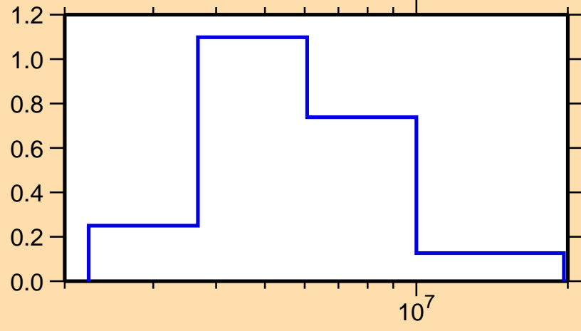
\sigma vs. E for ^{63}\text{Fe}(n,n\text{cont.})
