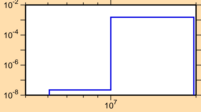
\sigma vs. E for ^{63}\text{Fe}(n,p)
