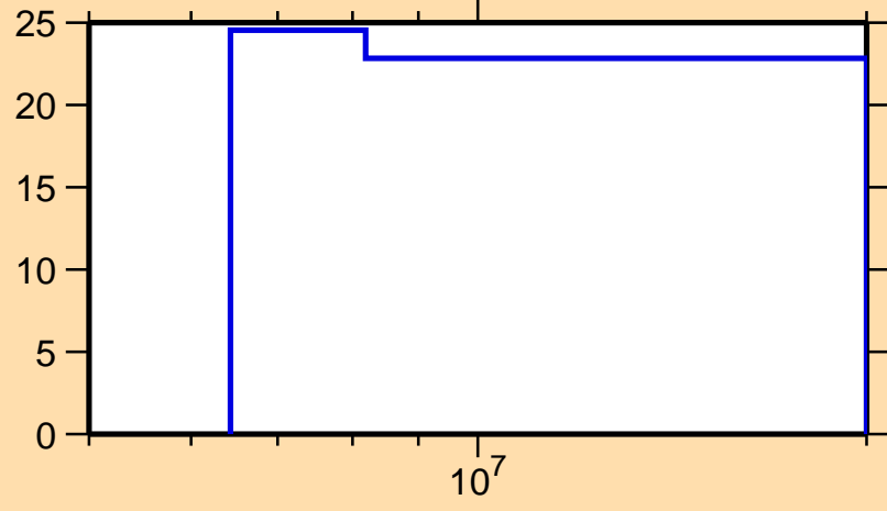
\Delta\sigma/\sigma vs. E for ^{63}\text{Fe}(n,el.)
