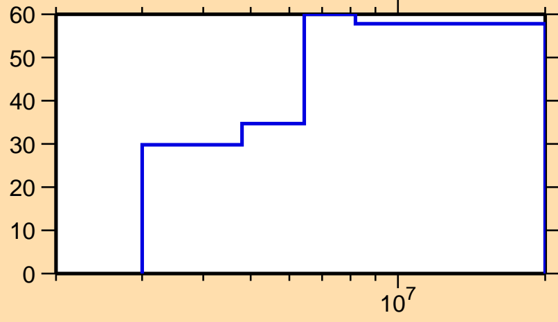
\Delta\sigma/\sigma vs. E for ^{63}\text{Fe}(n,n\text{cont.})
