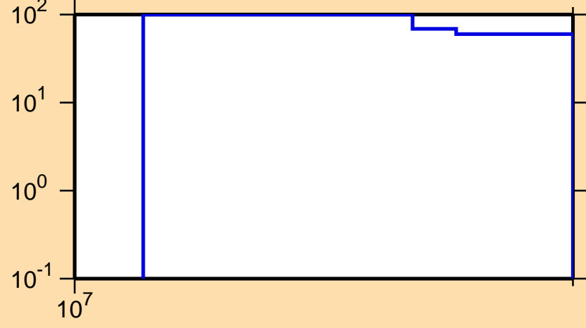
\Delta\sigma/\sigma vs. E for ^{64}\text{Fe}(n,p)
