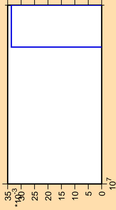
\Delta\sigma/\sigma vs. E for ^{64}\text{Fe}(n,nd)
