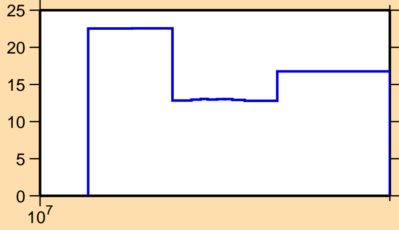
\Delta\sigma/\sigma vs. E for ^{64}\text{Fe}(n,el.)
