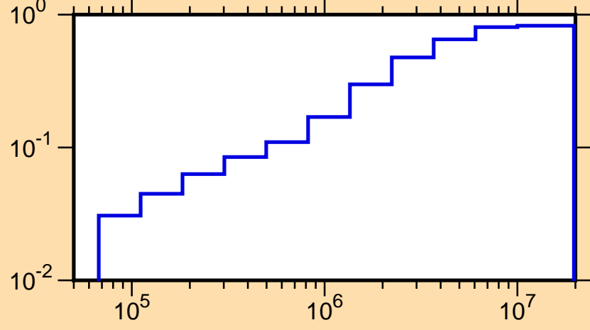
\mu vs. E for ^{64}\text{Fe}(\text{mt251})
