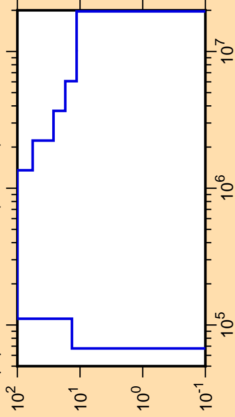
\Delta\mu/\mu vs. E for ^{64}\text{Fe}(\text{mt251})
