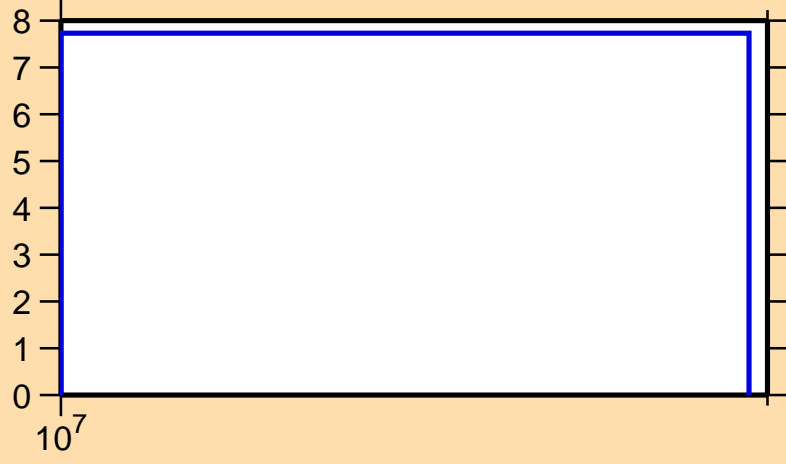
\Delta\sigma/\sigma vs. E for ^{64}\text{Fe}(n,\text{tot.})
