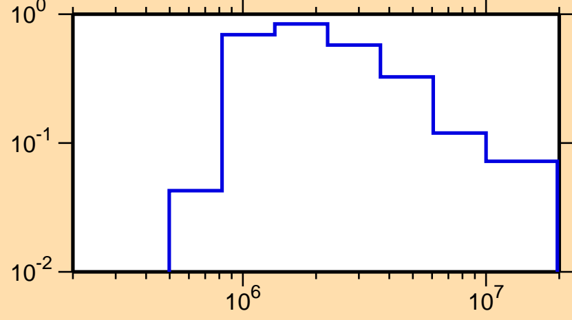
\sigma vs. E for ^{64}\text{Fe}(n,n_1)
