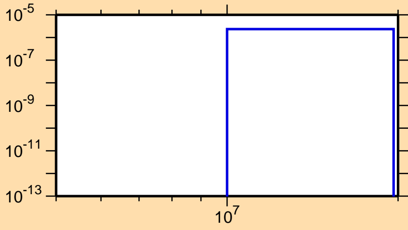
\sigma vs. E for ^{64}\text{Fe}(n,\alpha)
