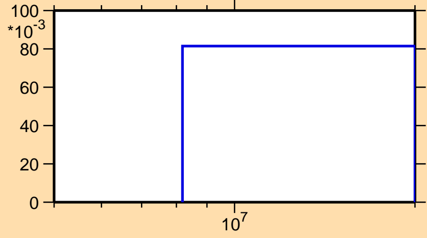
\sigma vs. E for ^{64}\text{Fe}(n,3n)
