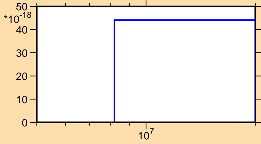
\sigma vs. E for ^{64}\text{Fe}(n,nd)
