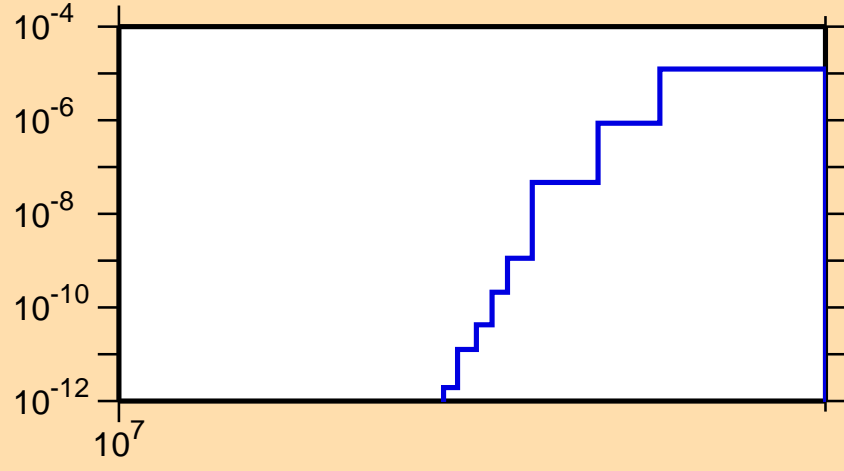
\sigma vs. E for ^{65}\text{Fe}(n,n\alpha)
