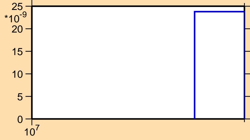
\sigma vs. E for ^{65}\text{Fe}(n,nd)
