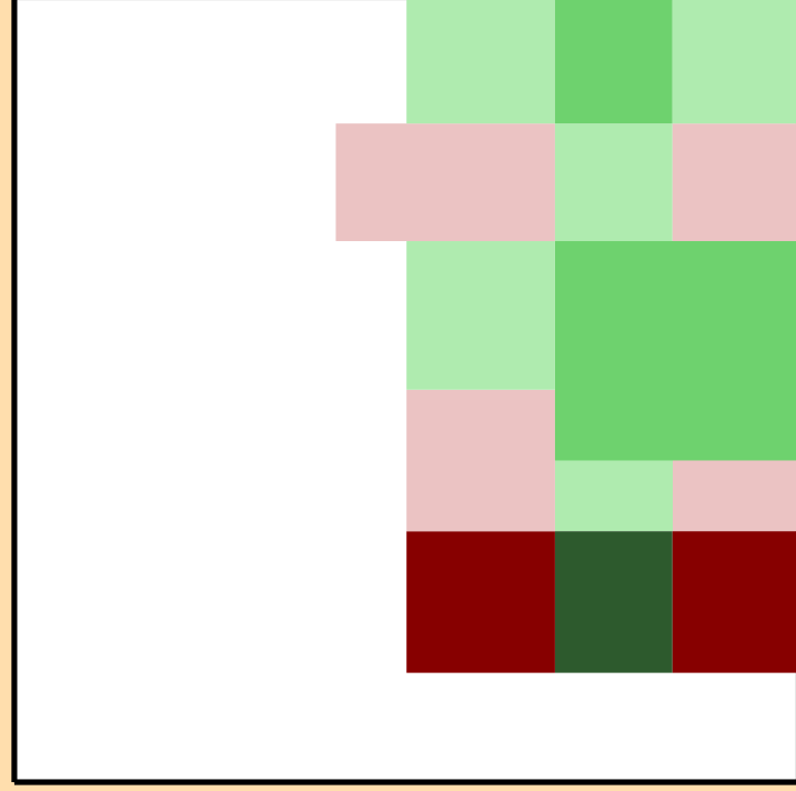
\Delta\sigma/\sigma vs. E for ^{65}\text{Fe}(n,p)
