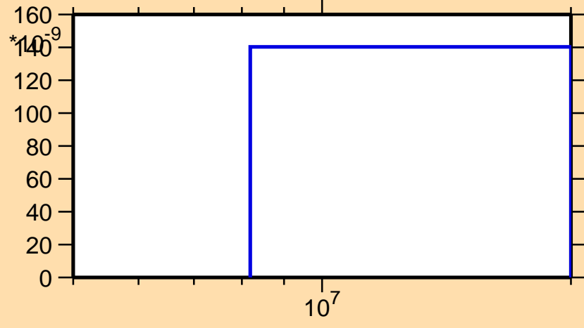
\sigma vs. E for ^{65}\text{Fe}(n,\alpha)
