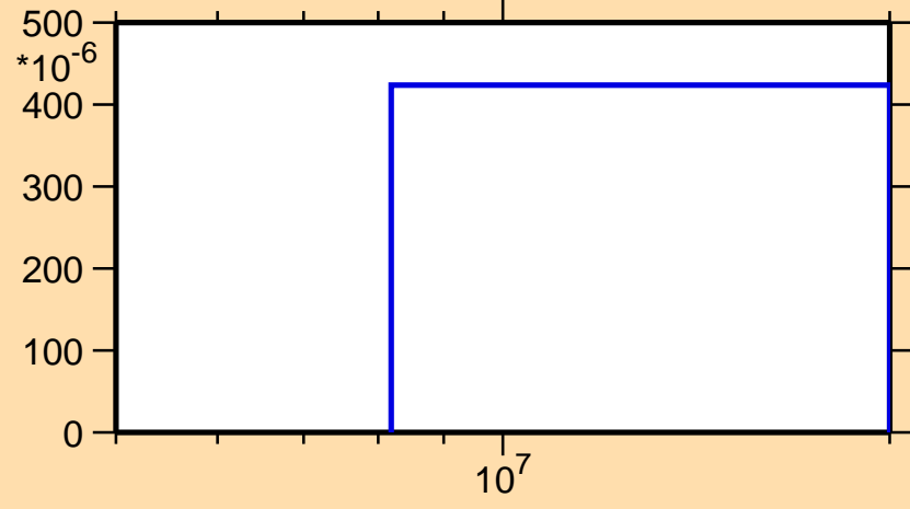
\sigma vs. E for ^{65}\text{Fe}(n,p)
