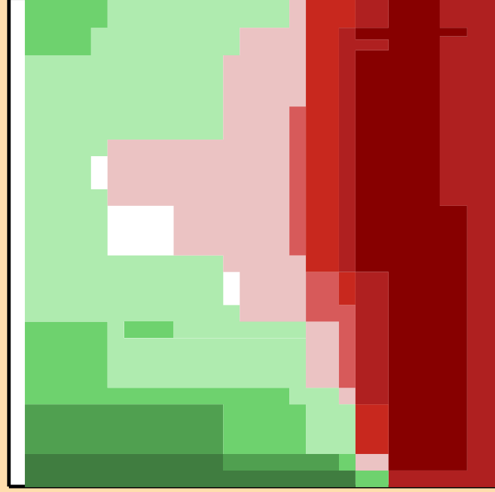
\Delta\sigma/\sigma vs. E for ^{204}\text{Fr}(n,n\text{cont.})
