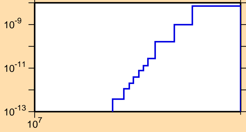
\sigma vs. E for ^{204}\text{Fr}(n,\text{pt})
