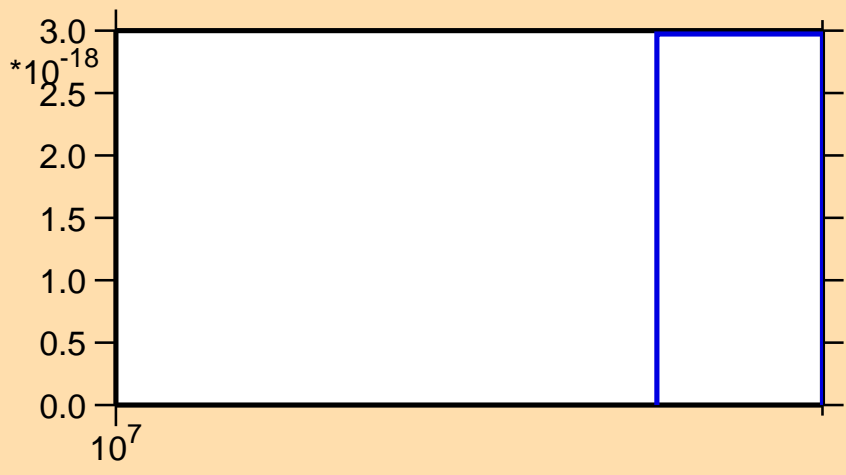
\sigma vs. E for ^{204}\text{Fr}(\text{mt } 42)
