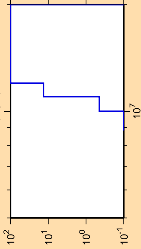
\Delta\sigma/\sigma vs. E for ^{204}\text{Fr}(n,pd)
