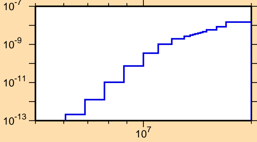
\sigma vs. E for ^{204}\text{Fr}(\text{mt117})
