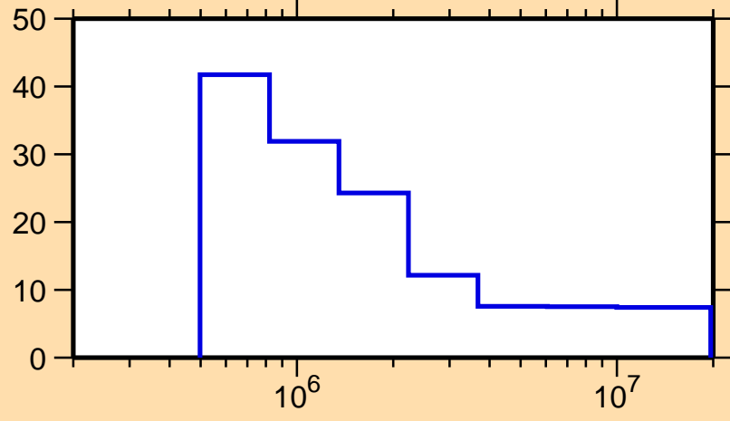
\Delta\sigma/\sigma vs. E for ^{204}\text{Fr}(n,n\text{onel.})
