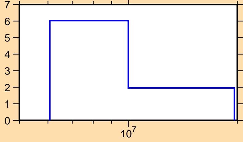
\Delta\sigma/\sigma vs. E for ^{204}\text{Fr}(n,\text{tot.})
