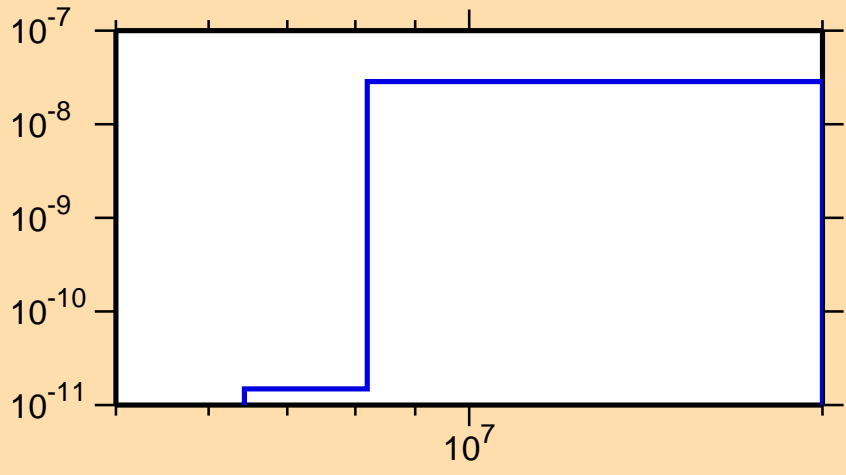
\sigma vs. E for ^{204}\text{Fr}(\text{mt } 45)
