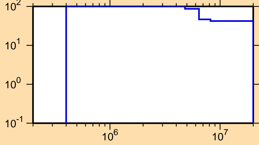
\Delta\sigma/\sigma vs. E for ^{204}\text{Fr}(n,n\text{cont.})
