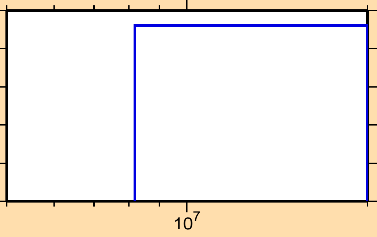
\sigma vs. E for ^{204}\text{Fr}(n,3n\alpha)
