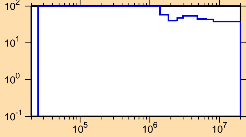
\Delta\sigma/\sigma vs. E for ^{204}\text{Fr}(n,n_1)
