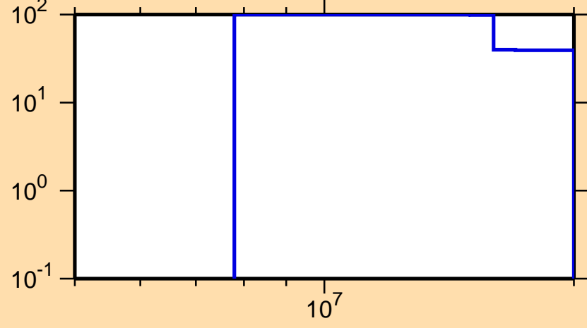
\Delta\sigma/\sigma vs. E for ^{204}\text{Fr}(n,2n)
