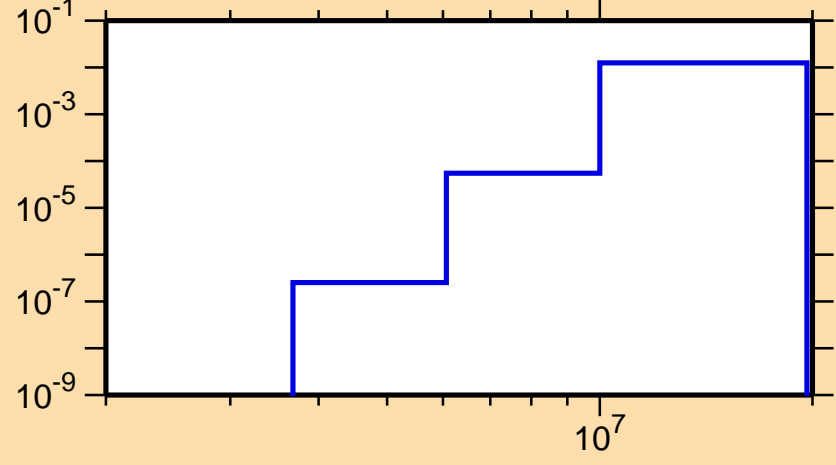
\sigma vs. E for ^{204}\text{Fr}(n,np)
