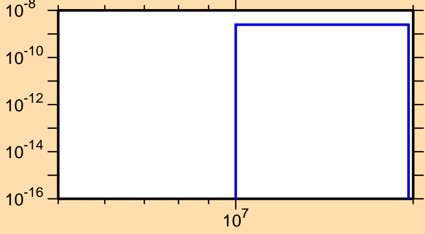
\sigma vs. E for ^{204}\text{Fr}(n,pd)
