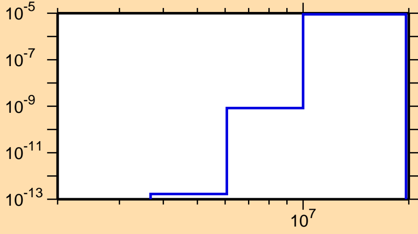
\sigma vs. E for ^{204}\text{Fr}(n,\text{He}3)
