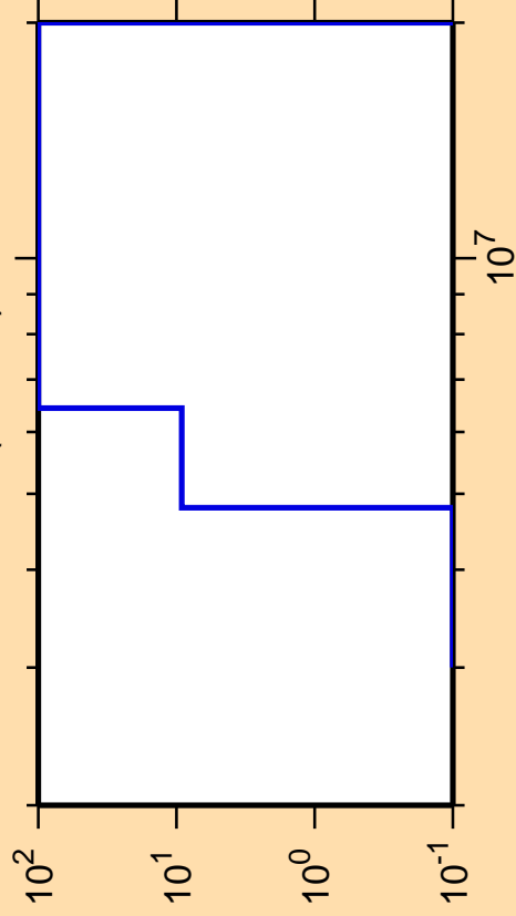
\Delta\sigma/\sigma vs. E for ^{204}\text{Fr}(n,\text{He}3)
