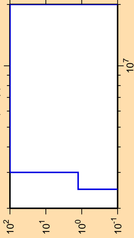
\Delta\sigma/\sigma vs. E for ^{204}\text{Fr}(n,np)
