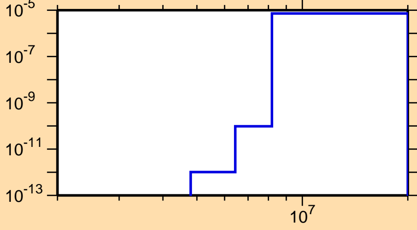
\sigma vs. E for ^{204}\text{Fr}(n,\text{He}3)
