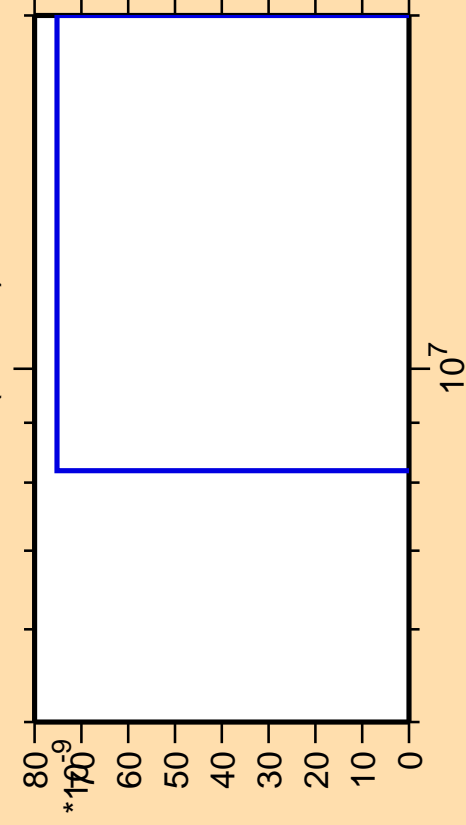
\Delta\sigma/\sigma vs. E for ^{204}\text{Fr}(\text{mt } 42)
