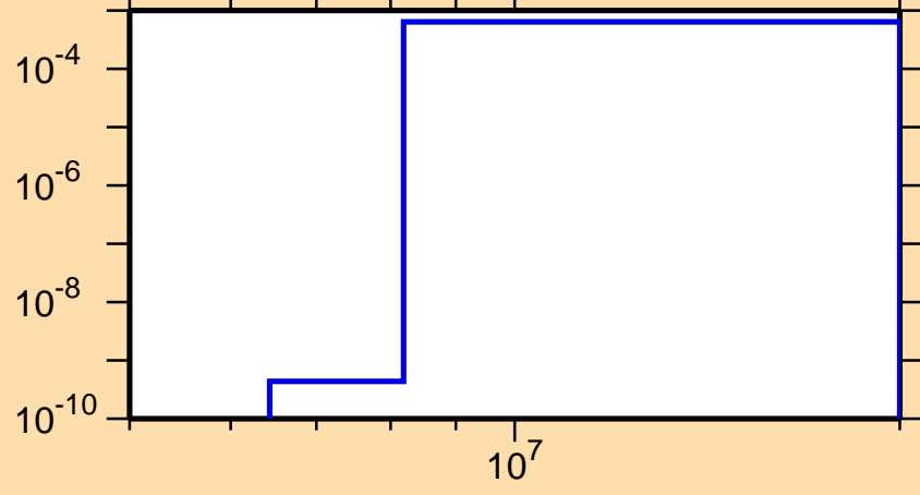
\sigma vs. E for ^{204}\text{Fr}(n,t)
