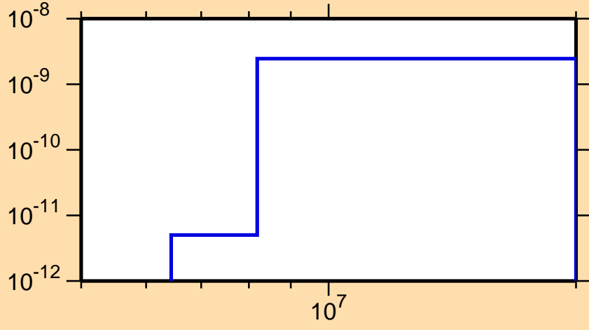
\sigma vs. E for ^{204}\text{Fr}(\text{mt117})
