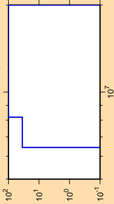
\Delta\sigma/\sigma vs. E for ^{204}\text{Fr}(\text{mt117})
