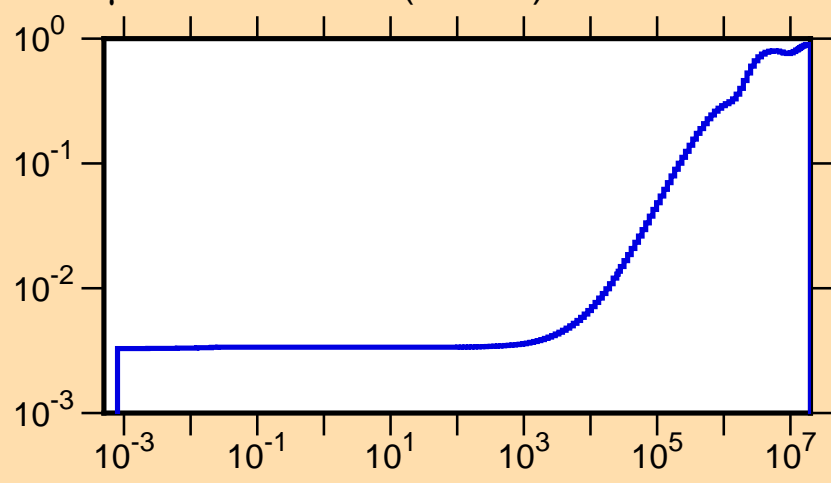
\mu vs. E for ^{205}\text{Fr}(\text{mt251})
