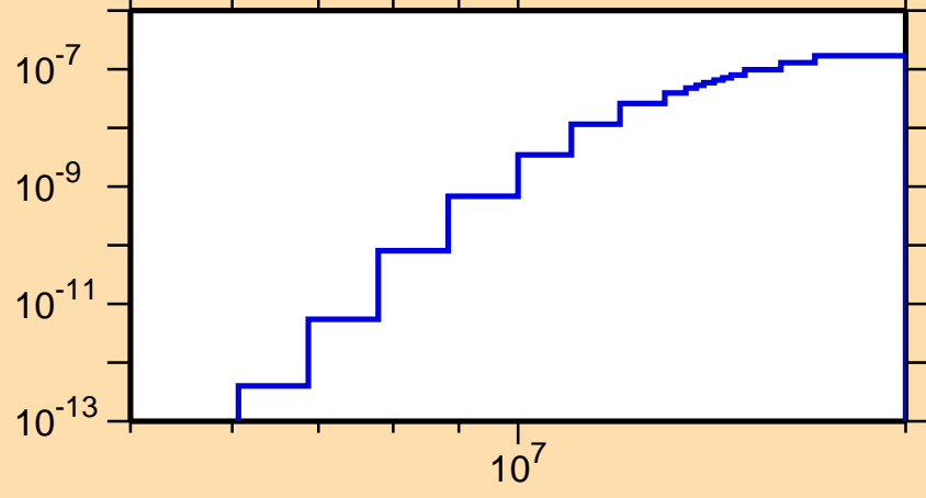
\sigma vs. E for ^{205}\text{Fr}(\text{mt117})
