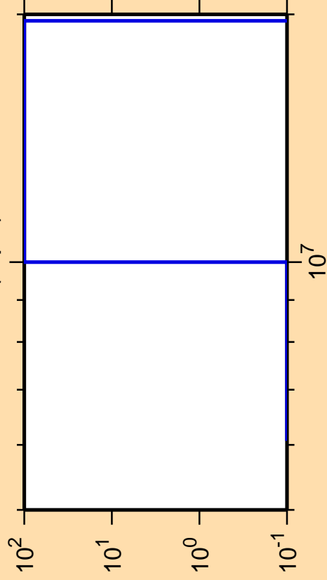
\Delta\sigma/\sigma vs. E for ^{205}\text{Fr}(n,pd)
