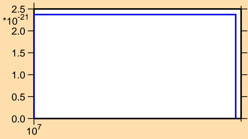
\sigma vs. E for ^{205}\text{Fr}(\text{mt } 42)
