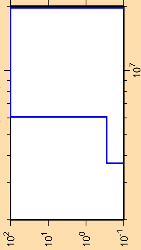
\Delta\sigma/\sigma vs. E for ^{205}\text{Fr}(\text{mt } 45)
