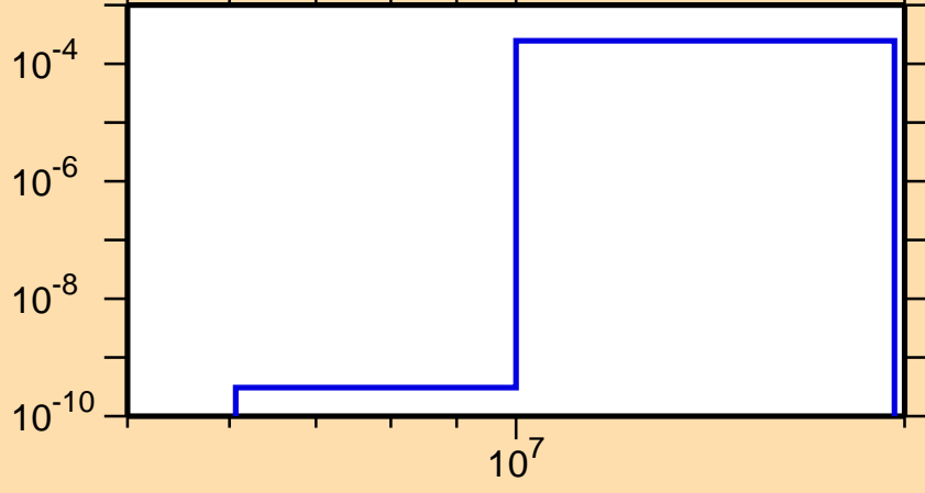
\sigma vs. E for ^{205}\text{Fr}(n,t)
