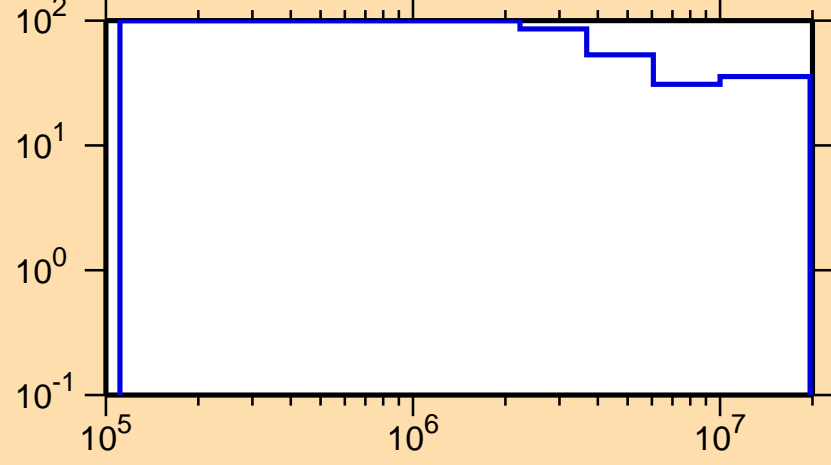
\Delta\sigma/\sigma vs. E for ^{205}\text{Fr}(n,n\text{cont.})
