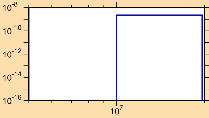
\sigma vs. E for ^{205}\text{Fr}(n,pd)
