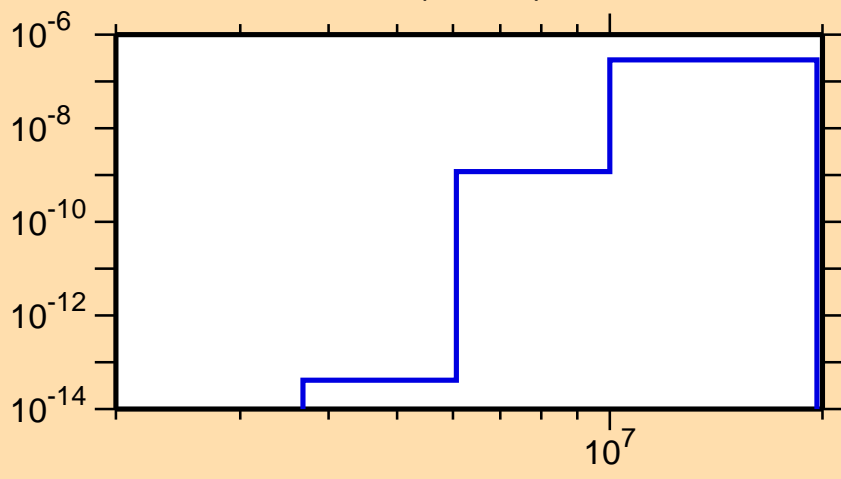
\sigma vs. E for ^{205}\text{Fr}(\text{mt } 45)
