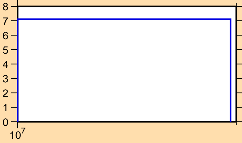
\Delta\sigma/\sigma vs. E for ^{205}\text{Fr}(n,\text{nonel.})
