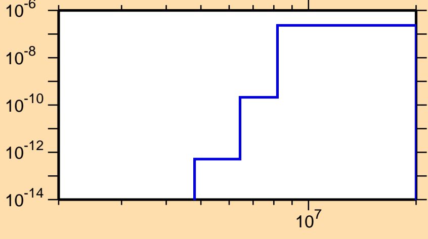
\sigma vs. E for ^{205}\text{Fr}(\text{mt } 45)
