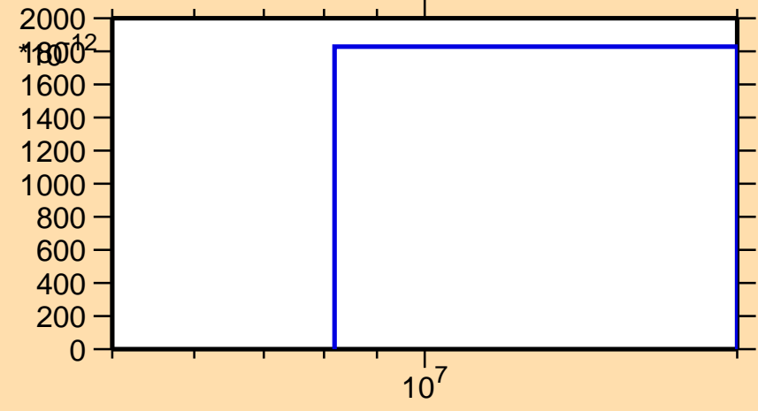
\sigma vs. E for ^{205}\text{Fr}(n,\text{pd})
