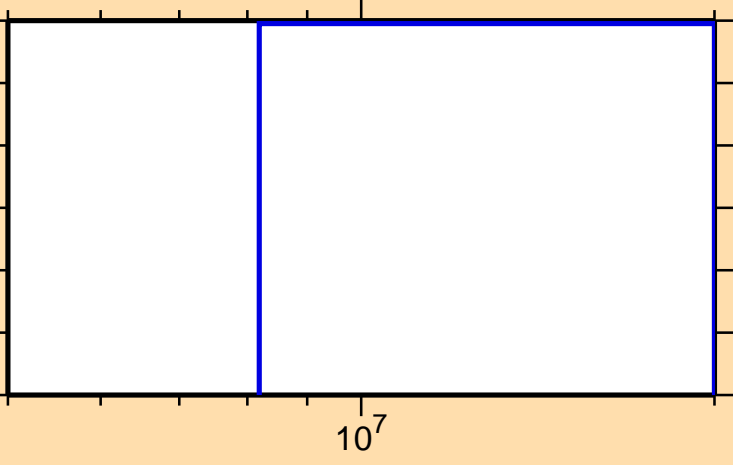
\sigma vs. E for ^{205}\text{Fr}(n,2n)
