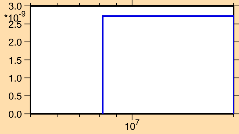
\sigma vs. E for ^{205}\text{Fr}(n,\text{nd})
