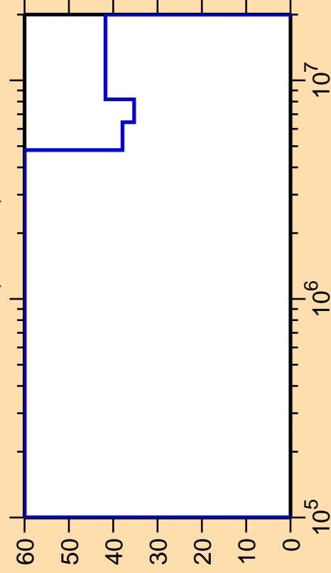
\Delta\sigma/\sigma vs. E for ^{205}\text{Fr}(n,\text{inel.})
