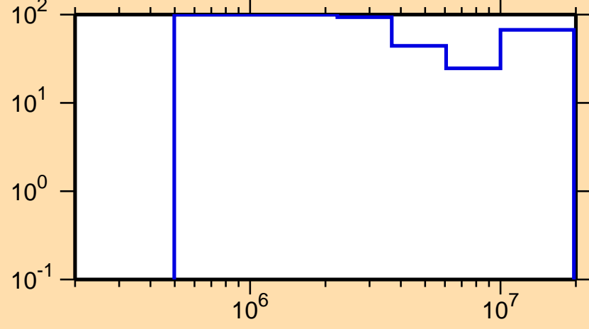
\Delta\sigma/\sigma vs. E for ^{206}\text{Fr}(n,ncont.)
