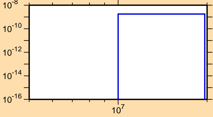
\sigma vs. E for ^{206}\text{Fr}(n,\text{pd})
