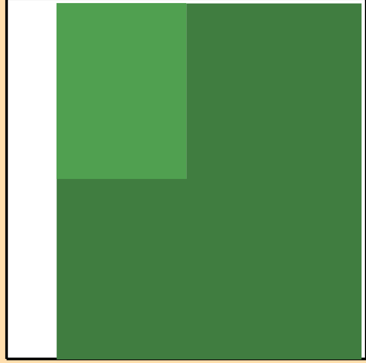
\Delta\sigma/\sigma vs. E for ^{206}\text{Fr}(n,2n)
