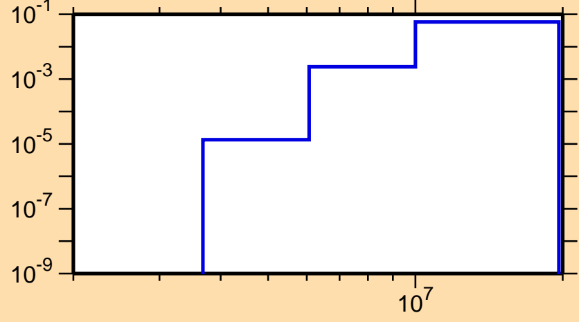
\sigma vs. E for ^{206}\text{Fr}(n,np)
