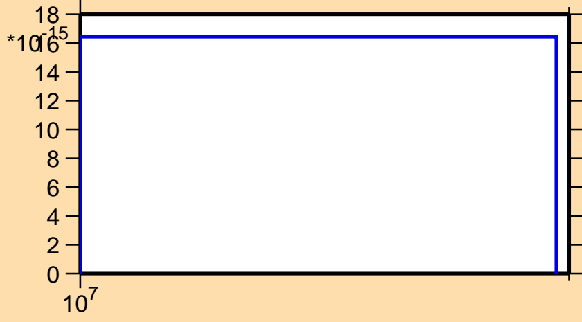
\sigma vs. E for ^{206}\text{Fr}(n,3n\alpha)
