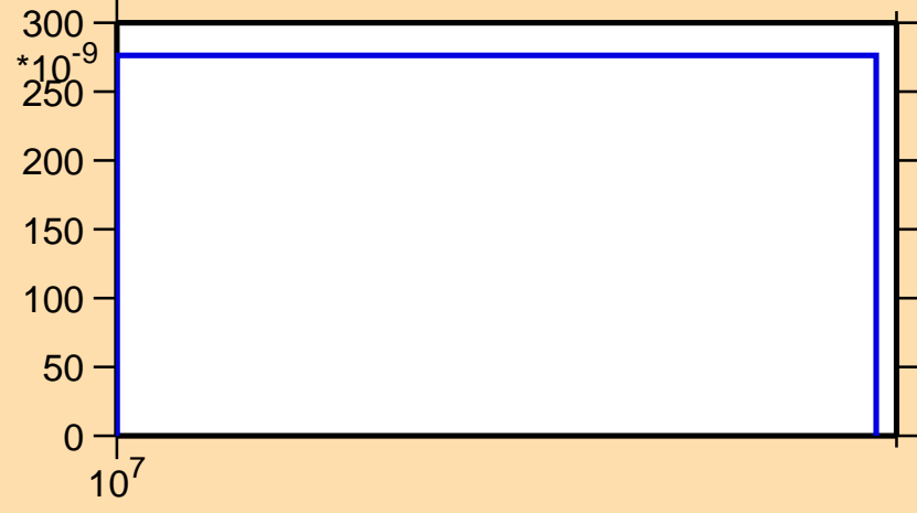
\sigma vs. E for ^{206}\text{Fr}(n,3n)
