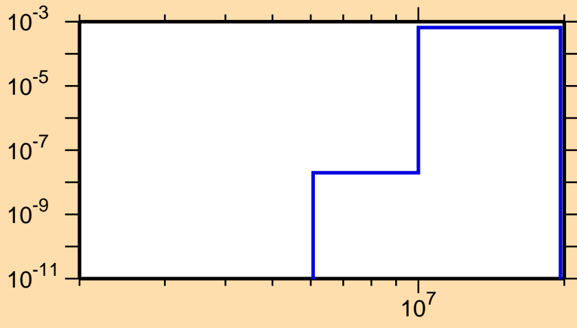
\sigma vs. E for ^{206}\text{Fr}(n,t)
