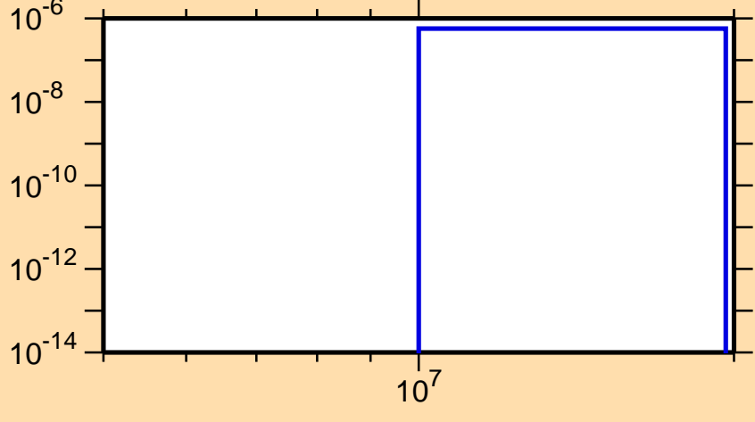
\sigma vs. E for ^{206}\text{Fr}(n,\text{nd})
