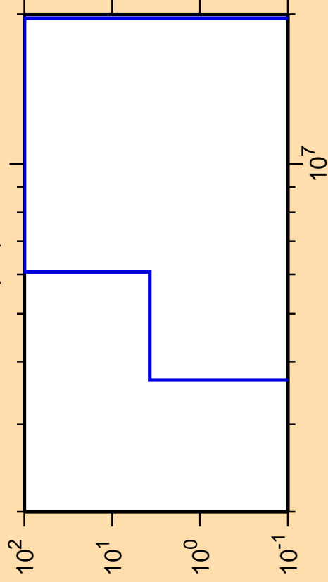
\Delta\sigma/\sigma vs. E for ^{206}\text{Fr}(n,t)
