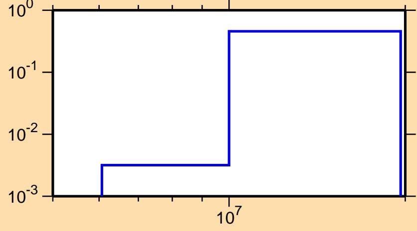
\sigma vs. E for ^{206}\text{Fr}(n,2n)
