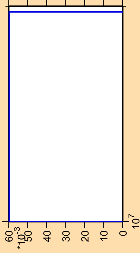
\Delta\sigma/\sigma vs. E for ^{206}\text{Fr}(n,3n\alpha)
