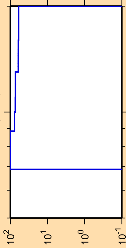
\Delta\sigma/\sigma vs. E for ^{206}\text{Fr}(n,2n)
