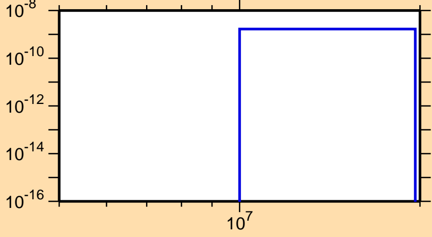
\sigma vs. E for ^{206}\text{Fr}(n,pd)
