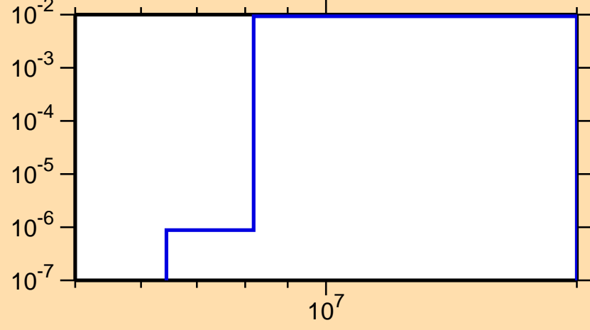
\sigma vs. E for ^{206}\text{Fr}(n,2n\alpha)
