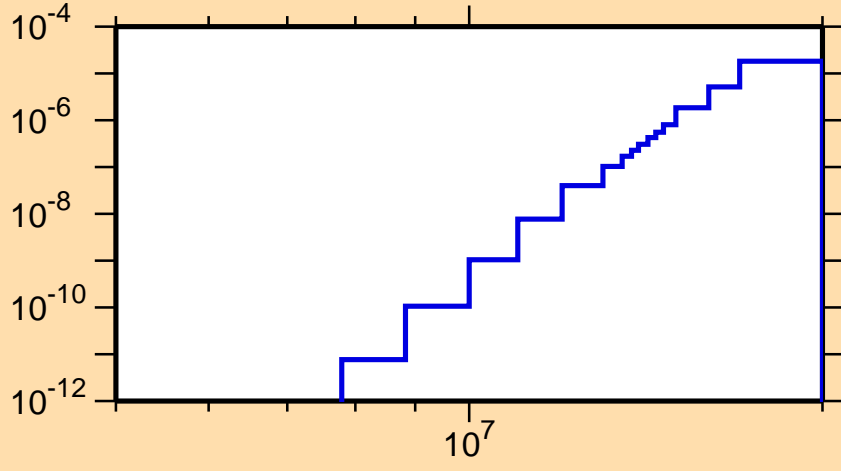
\sigma vs. E for ^{207}\text{Fr}(n,\text{He}3)
