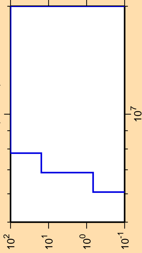
\Delta\sigma/\sigma vs. E for ^{207}\text{Fr}(\text{mt117})
