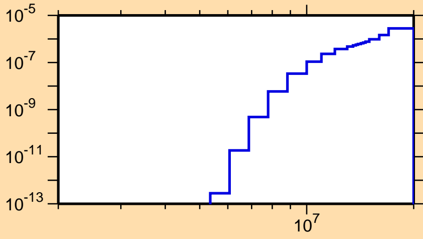
\sigma vs. E for ^{207}\text{Fr}(\text{mt } 45)
