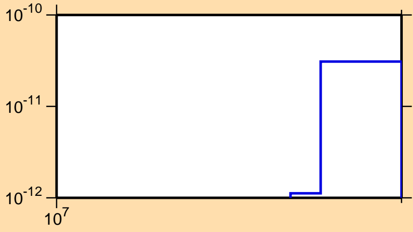
\sigma vs. E for ^{207}\text{Fr}(\text{mt } 34)
