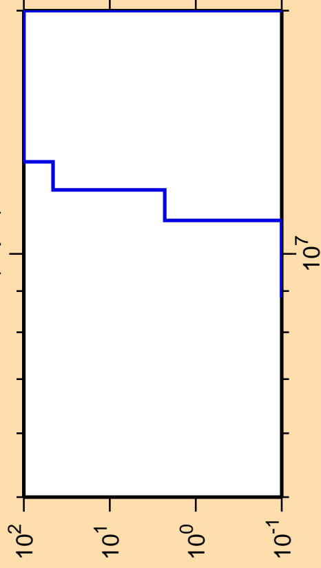
\Delta\sigma/\sigma vs. E for ^{207}\text{Fr}(n,pd)
