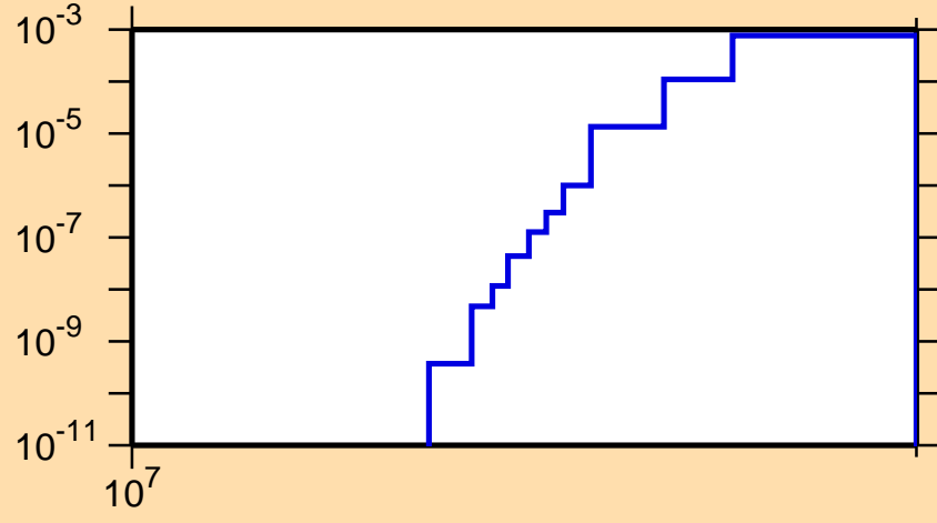
\sigma vs. E for ^{207}\text{Fr}(n,2np)
