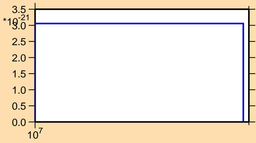
\sigma vs. E for ^{207}\text{Fr}(\text{mt } 42)
