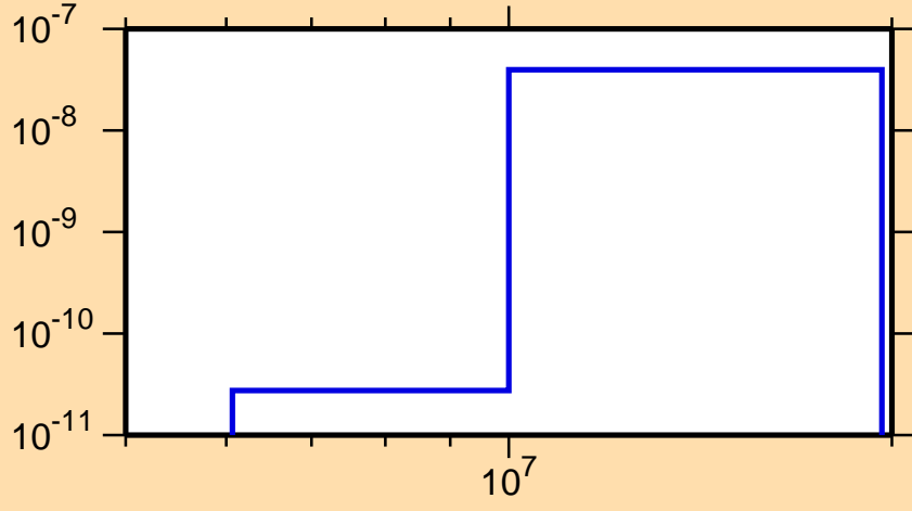
\sigma vs. E for ^{207}\text{Fr}(\text{mt117})
