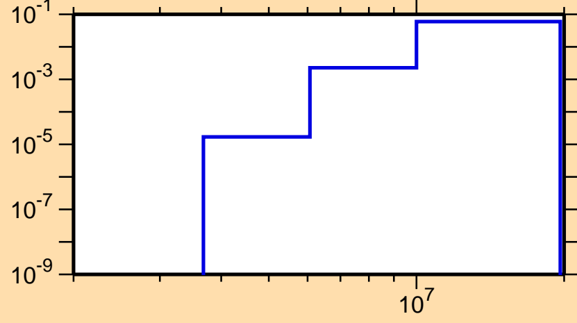
\sigma vs. E for ^{207}\text{Fr}(n,np)
