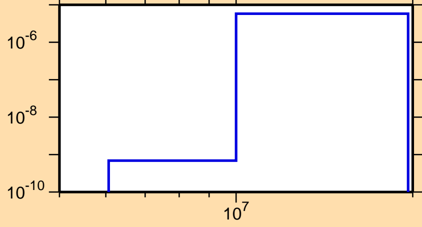
\sigma vs. E for ^{207}\text{Fr}(n,2n\alpha)
