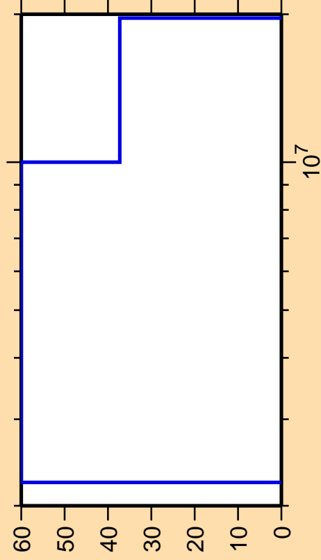
\Delta\sigma/\sigma vs. E for ^{207}\text{Fr}(n,np)
