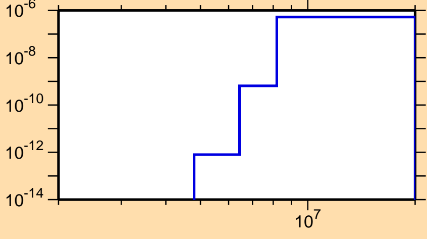
\sigma vs. E for ^{207}\text{Fr}(\text{mt } 45)
