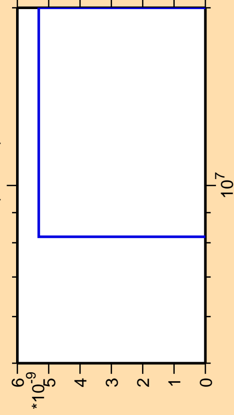
\Delta\sigma/\sigma vs. E for ^{207}\text{Fr}(\text{mt } 42)
