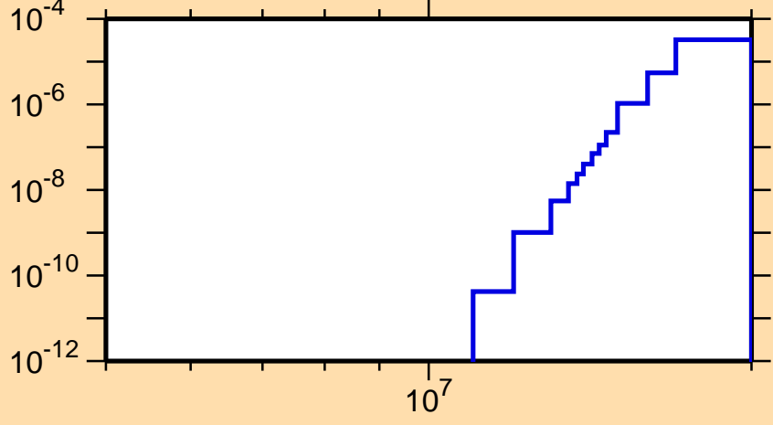
\sigma vs. E for ^{208}\text{Fr}(n,\text{nd})
