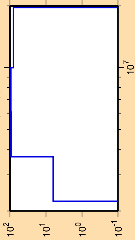
\Delta\sigma/\sigma vs. E for ^{208}\text{Fr}(n,np)
