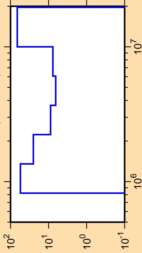
\Delta\sigma/\sigma vs. E for ^{208}\text{Fr}(n,\text{ncont.})
