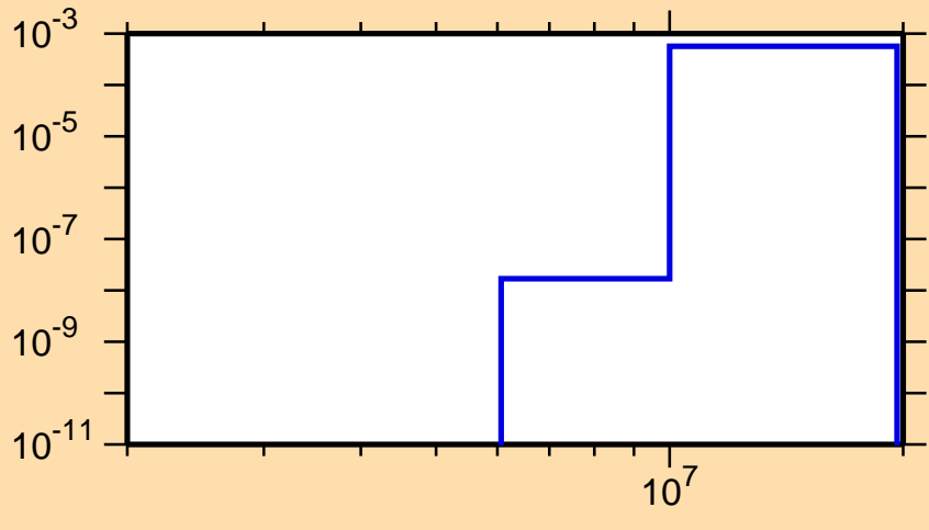
\sigma vs. E for ^{208}\text{Fr}(n,t)
