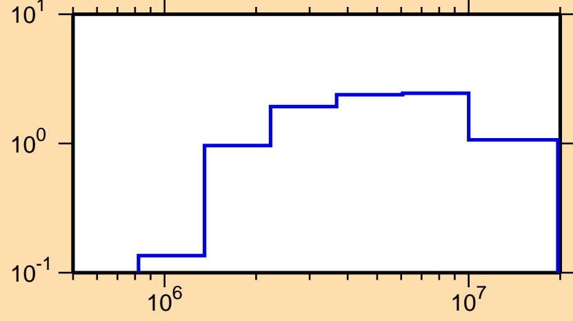
\sigma vs. E for ^{208}\text{Fr}(n,n\text{cont.})
