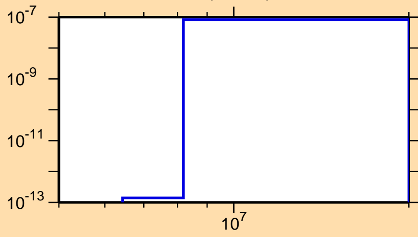
\sigma vs. E for ^{208}\text{Fr}(\text{mt } 45)
