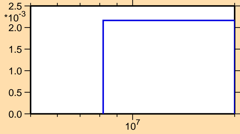
\sigma vs. E for ^{208}\text{Fr}(n,2n\alpha)
