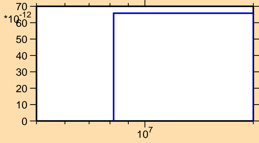
\sigma vs. E for ^{208}\text{Fr}(n,3n\alpha)
