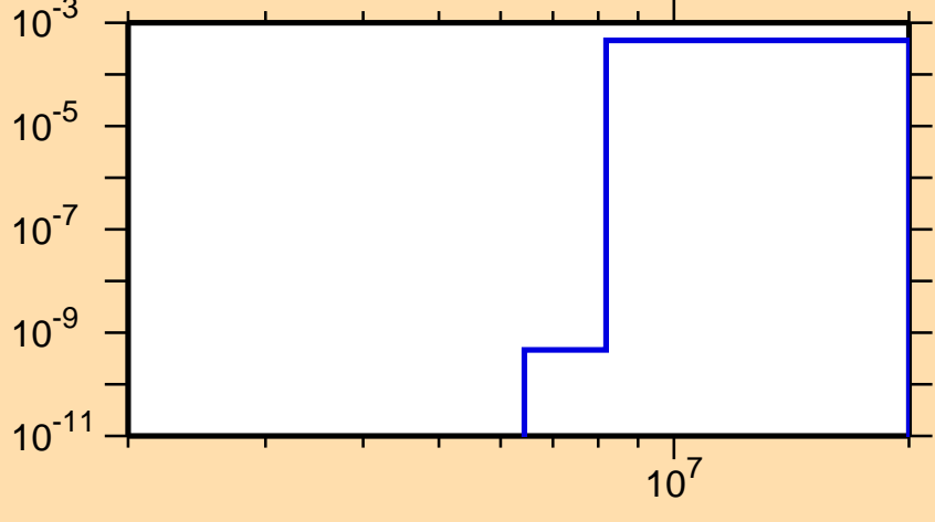
\sigma vs. E for ^{208}\text{Fr}(n,t)
