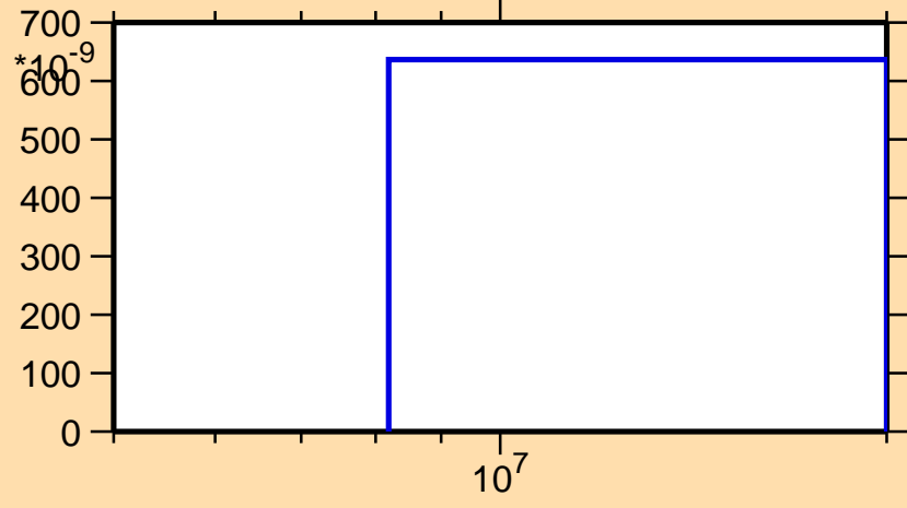
\sigma vs. E for ^{208}\text{Fr}(n,\text{nd})
