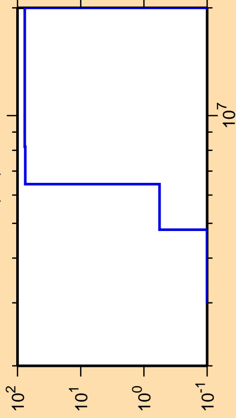
\Delta\sigma/\sigma vs. E for ^{208}\text{Fr}(n,t)
