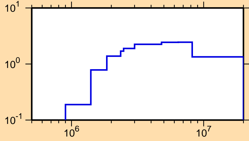
\sigma vs. E for ^{208}\text{Fr}(n,n\text{cont.})
