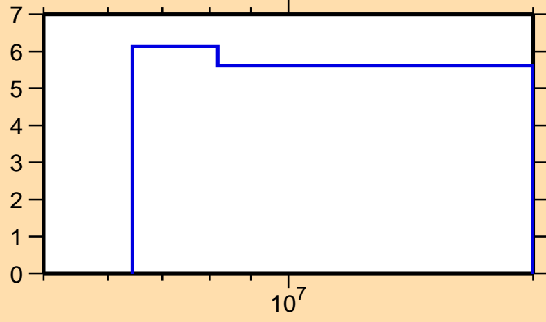
\Delta\sigma/\sigma vs. E for ^{208}\text{Fr}(n,\text{nonel.})
