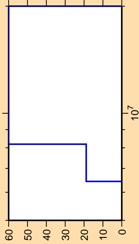
\Delta\sigma/\sigma vs. E for ^{208}\text{Fr}(n,\text{He}3)
