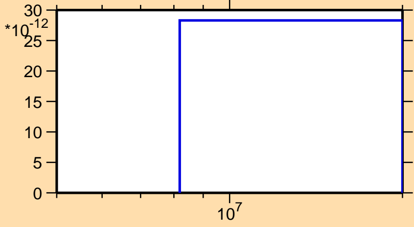
\sigma vs. E for ^{208}\text{Fr}(\text{mt } 34)
