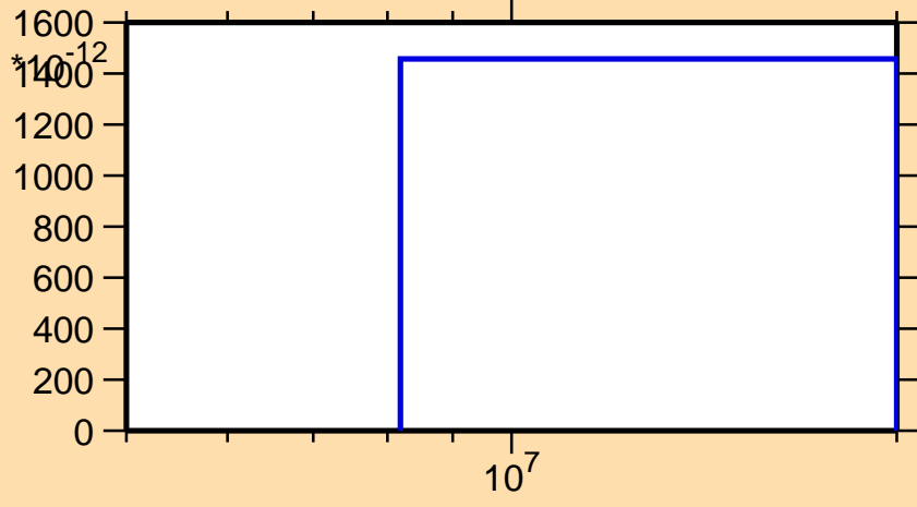
\sigma vs. E for ^{208}\text{Fr}(\text{mt117})
