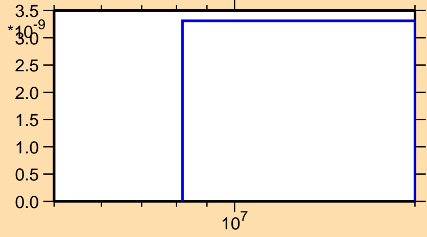
\sigma vs. E for ^{208}\text{Fr}(n,\text{pd})
