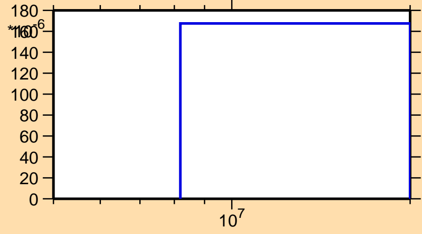
\sigma vs. E for ^{208}\text{Fr}(n,2np)
