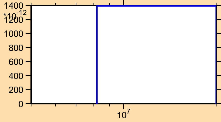
\sigma vs. E for ^{208}\text{Fr}(n,nt)
