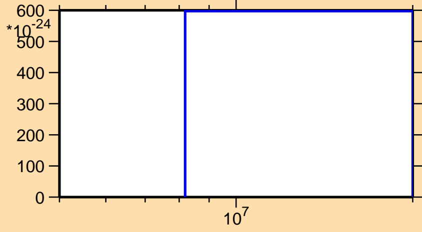
\sigma vs. E for ^{208}\text{Fr}(\text{mt } 42)
