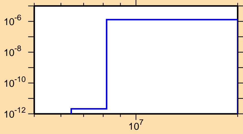
\sigma vs. E for ^{208}\text{Fr}(n,\text{He}3)
