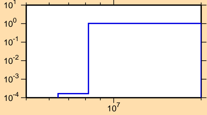
\sigma vs. E for ^{208}\text{Fr}(n,2n)
