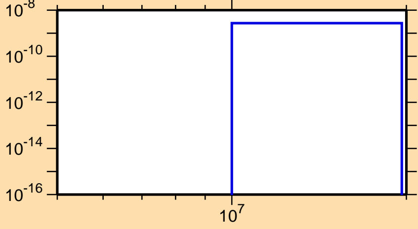
\sigma vs. E for ^{209}\text{Fr}(n,pd)
