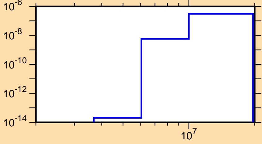
\sigma vs. E for ^{209}\text{Fr}(\text{mt } 45)
