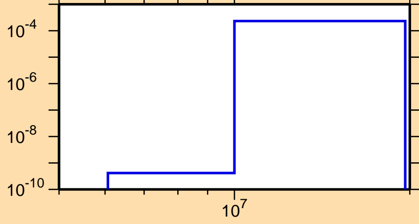
\sigma vs. E for ^{209}\text{Fr}(n,t)
