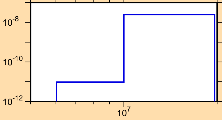
\sigma vs. E for ^{209}\text{Fr}(\text{mt117})
