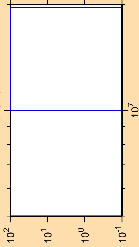
\Delta\sigma/\sigma vs. E for ^{209}\text{Fr}(n,pd)
