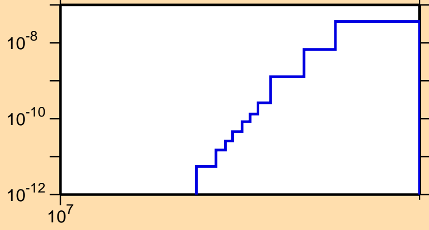
\sigma vs. E for ^{210}\text{Fr}(n,pd)
