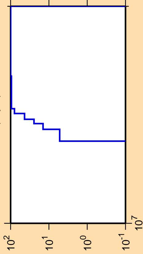
\Delta\sigma/\sigma vs. E for ^{210}\text{Fr}(n,pd)
