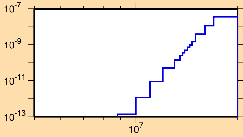
\sigma vs. E for ^{210}\text{Fr}(\text{mt117})
