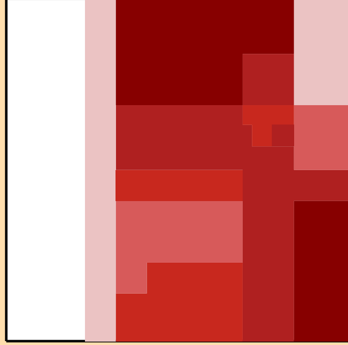
\Delta\sigma/\sigma vs. E for ^{210}\text{Fr}(n,2n)
