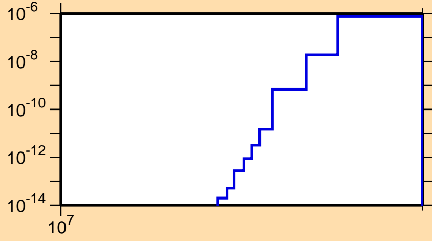
\sigma vs. E for ^{210}\text{Fr}(n,nt)
