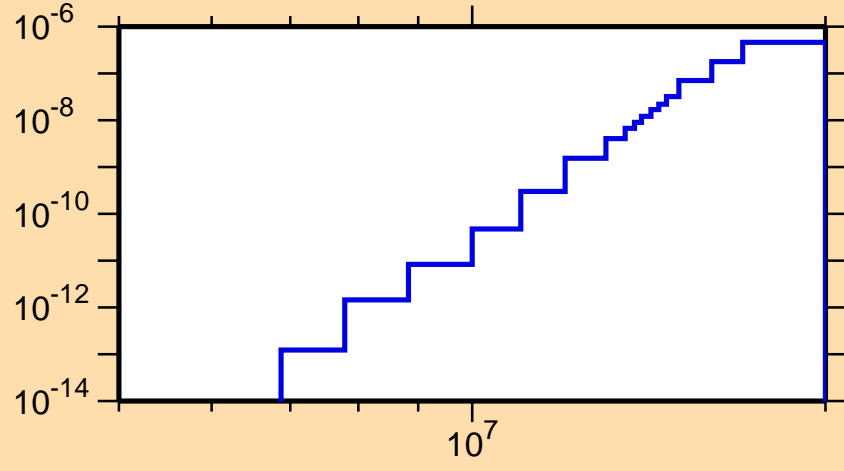
\sigma vs. E for ^{210}\text{Fr}(\text{mt } 45)
