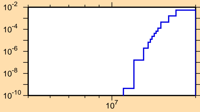
\sigma vs. E for ^{210}\text{Fr}(n,2np)
