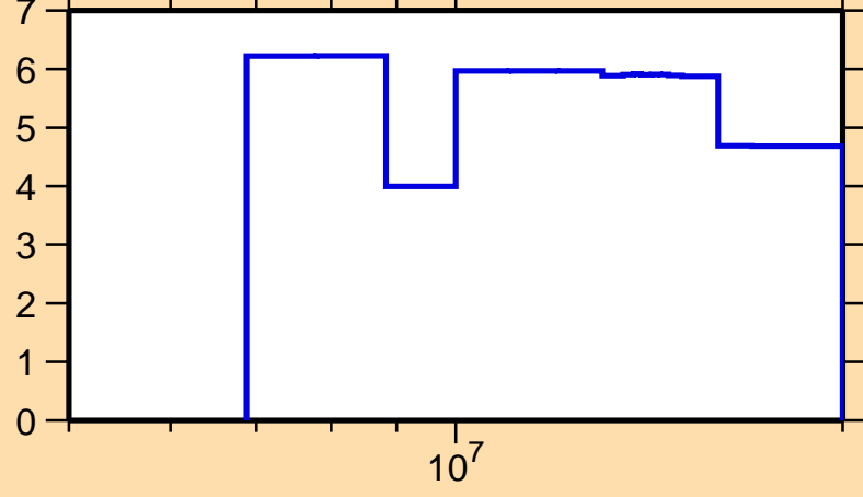
\Delta\sigma/\sigma vs. E for ^{210}\text{Fr}(n,\text{el.})
