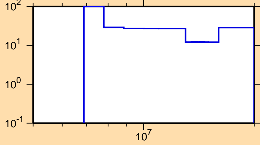
\Delta\sigma/\sigma vs. E for ^{210}\text{Fr}(n,2n)
