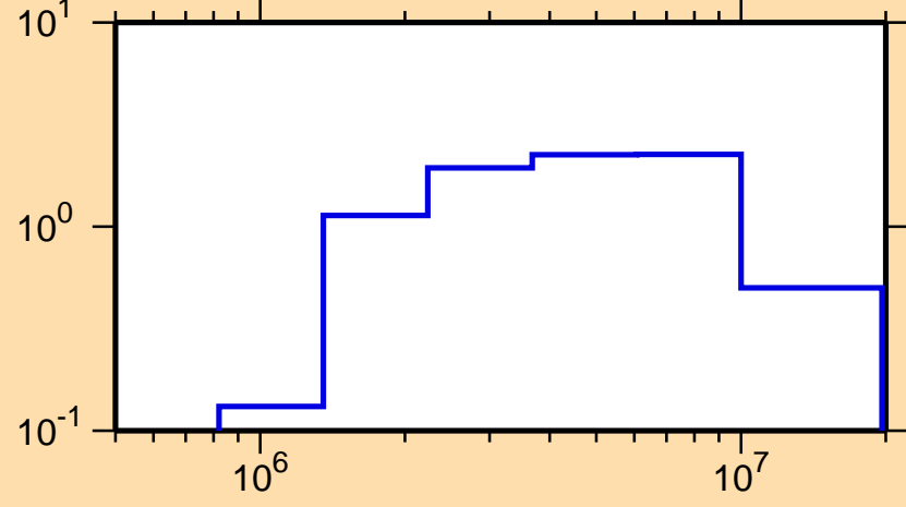
\sigma vs. E for ^{210}\text{Fr}(n,n\text{cont.})
