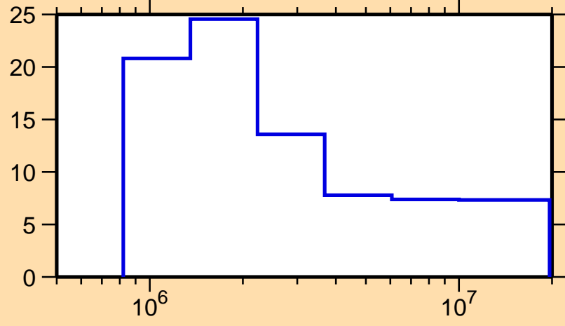
\Delta\sigma/\sigma vs. E for ^{210}\text{Fr}(n,n\text{onel.})
