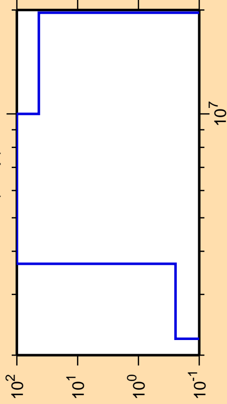
\Delta\sigma/\sigma vs. E for ^{210}\text{Fr}(n,np)
