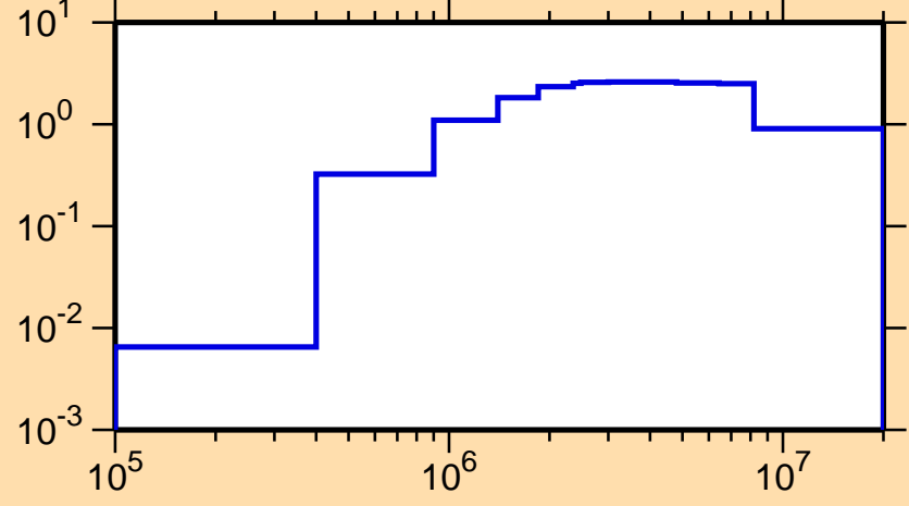
\sigma vs. E for ^{210}\text{Fr}(n,\text{inel.})
