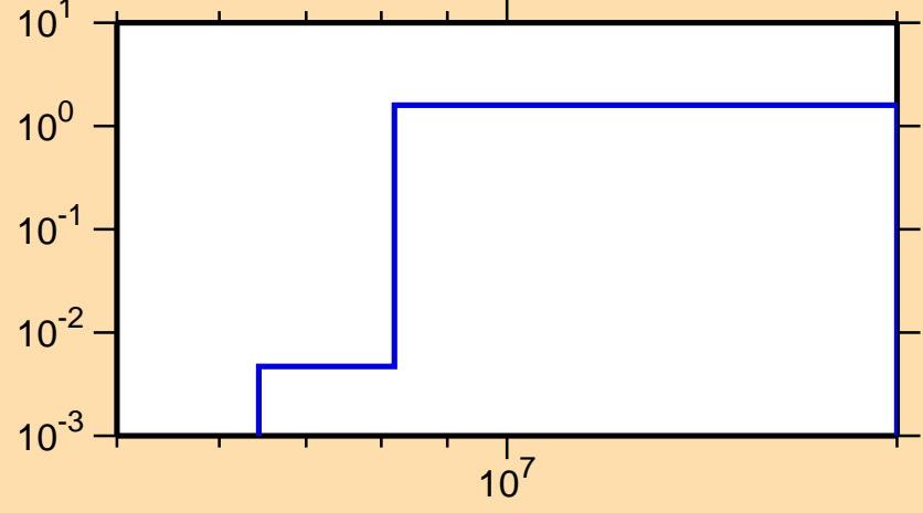
\sigma vs. E for ^{210}\text{Fr}(n,2n)
