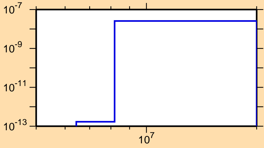
\sigma vs. E for ^{210}\text{Fr}(\text{mt } 45)
