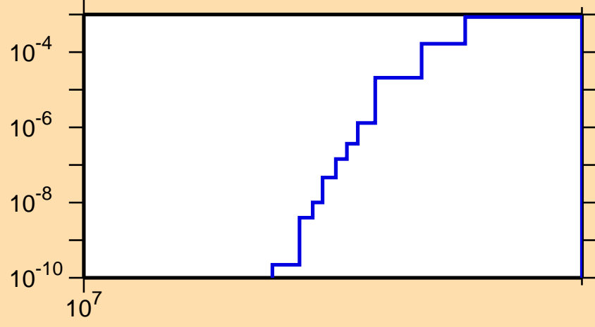
\sigma vs. E for ^{211}\text{Fr}(n,2np)
