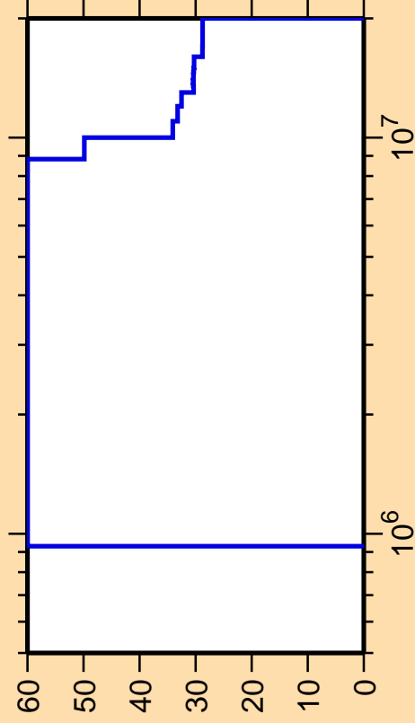
\Delta\sigma/\sigma vs. E for ^{211}\text{Fr}(n,p\alpha)
