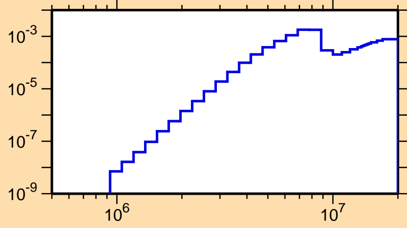
\sigma vs. E for ^{211}\text{Fr}(n,p\alpha)
