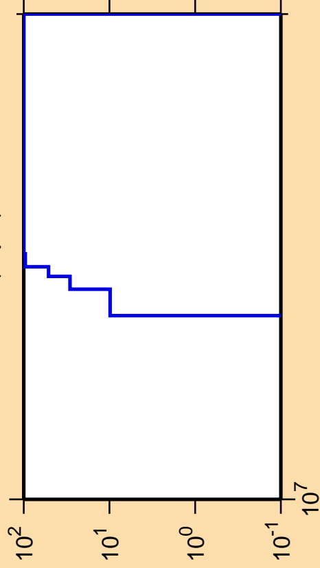
\Delta\sigma/\sigma vs. E for ^{211}\text{Fr}(n,pd)
