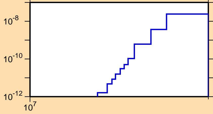
\sigma vs. E for ^{211}\text{Fr}(n,pd)
