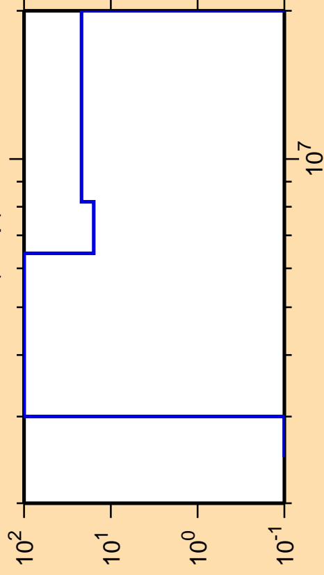
\Delta\sigma/\sigma vs. E for ^{211}\text{Fr}(n,np)
