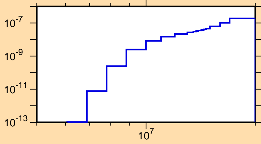
\sigma vs. E for ^{212}\text{Fr}(\text{mt } 45)
