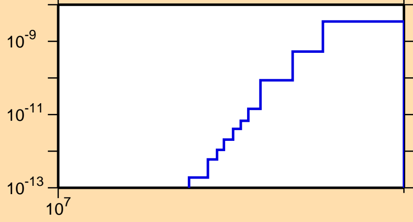
\sigma vs. E for ^{212}\text{Fr}(n,pd)
