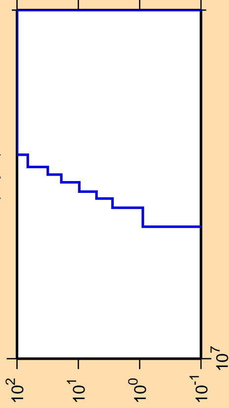
\Delta\sigma/\sigma vs. E for ^{212}\text{Fr}(n,pd)
