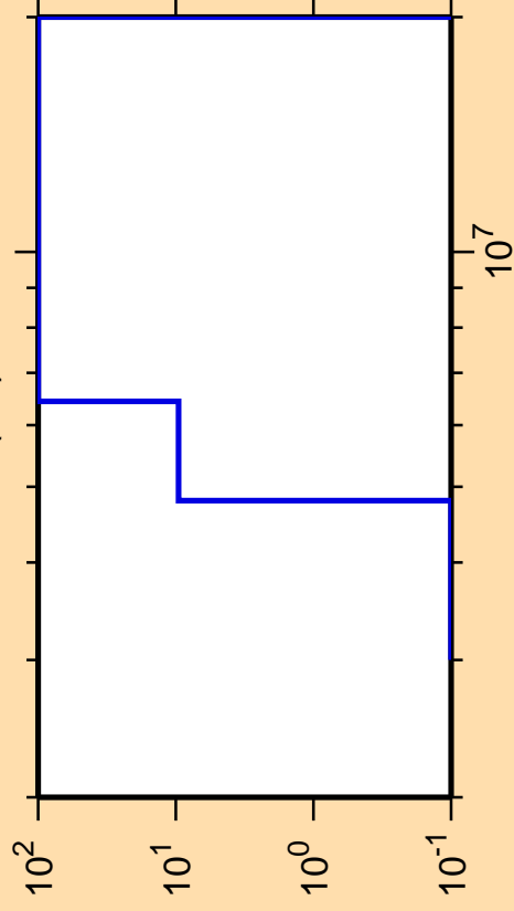
\Delta\sigma/\sigma vs. E for ^{212}\text{Fr}(n,t)
