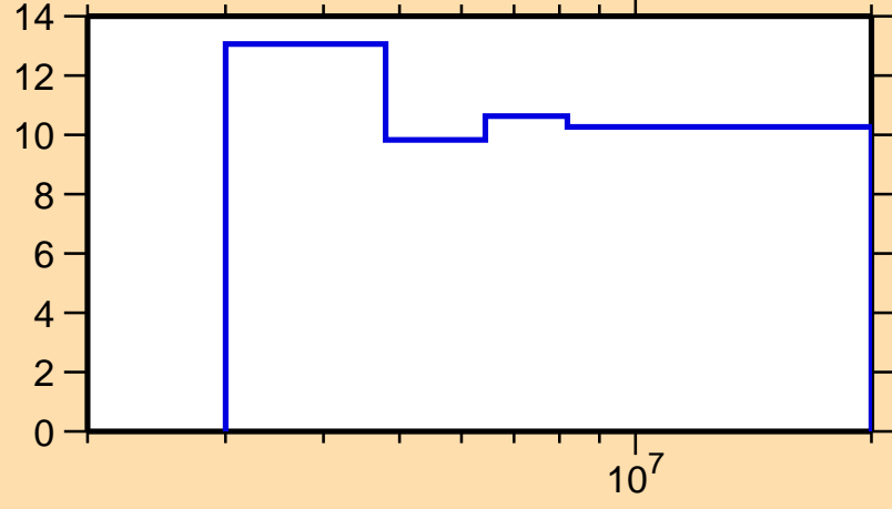
\Delta\sigma/\sigma vs. E for ^{212}\text{Fr}(n,n\text{onel.})
