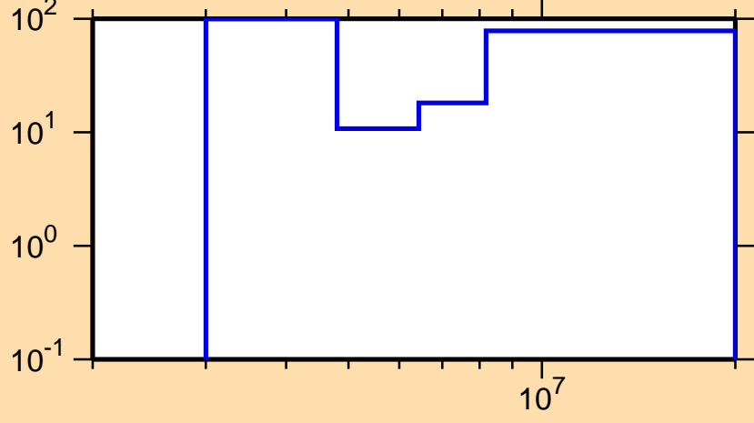
\Delta\sigma/\sigma vs. E for ^{212}\text{Fr}(n,n\text{cont.})
