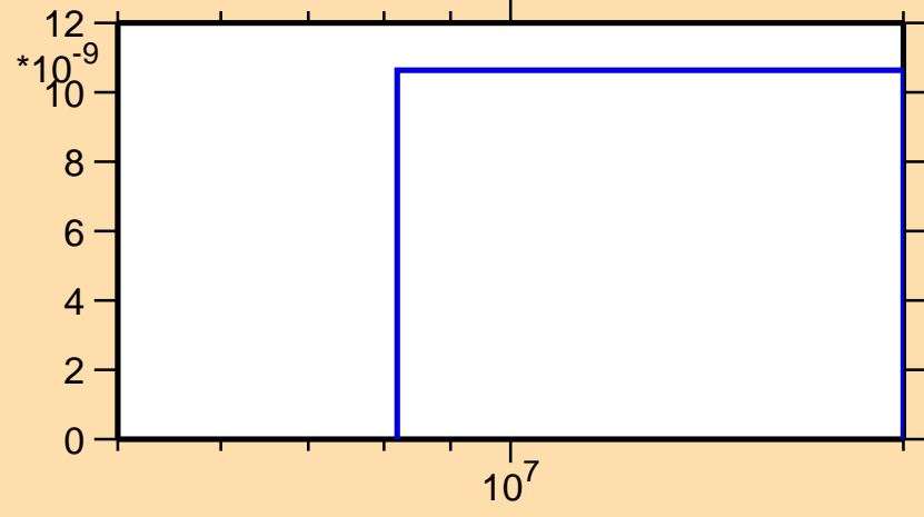
\sigma vs. E for ^{212}\text{Fr}(n,nt)
