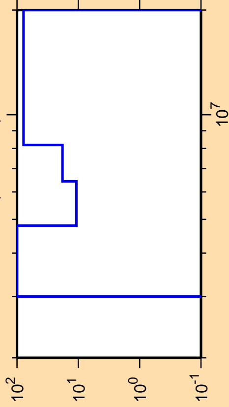
\Delta\sigma/\sigma vs. E for ^{212}\text{Fr}(n,\text{ncont.})
