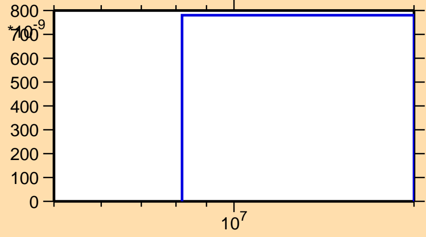
\sigma vs. E for ^{212}\text{Fr}(n,\text{nd})
