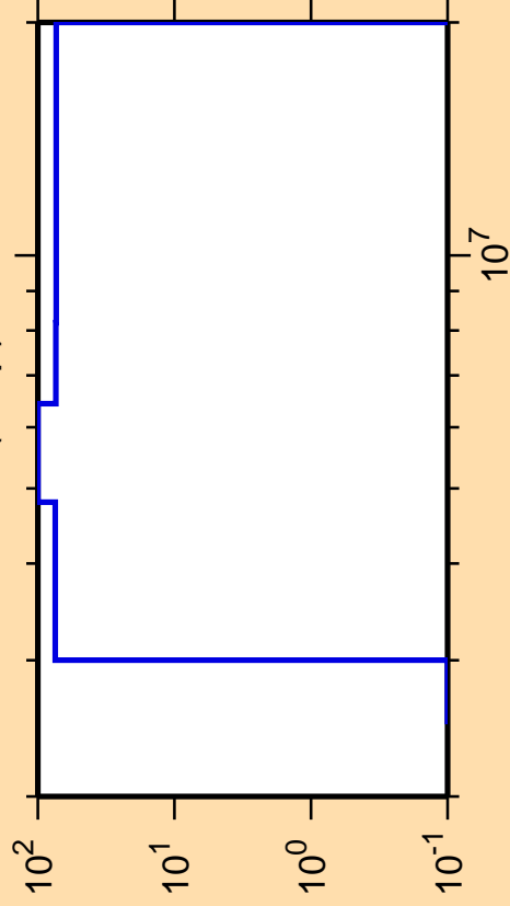
\Delta\sigma/\sigma vs. E for ^{212}\text{Fr}(n,np)
