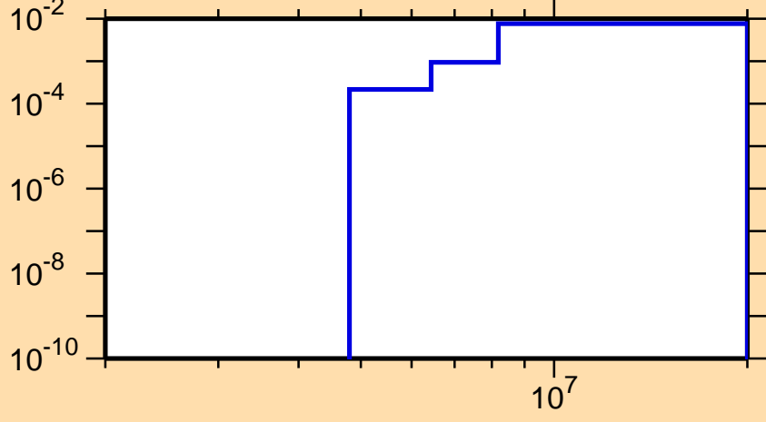
\sigma vs. E for ^{212}\text{Fr}(n,np)
