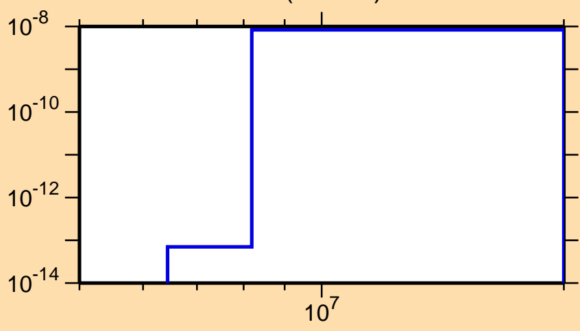
\sigma vs. E for ^{212}\text{Fr}(\text{mt117})
