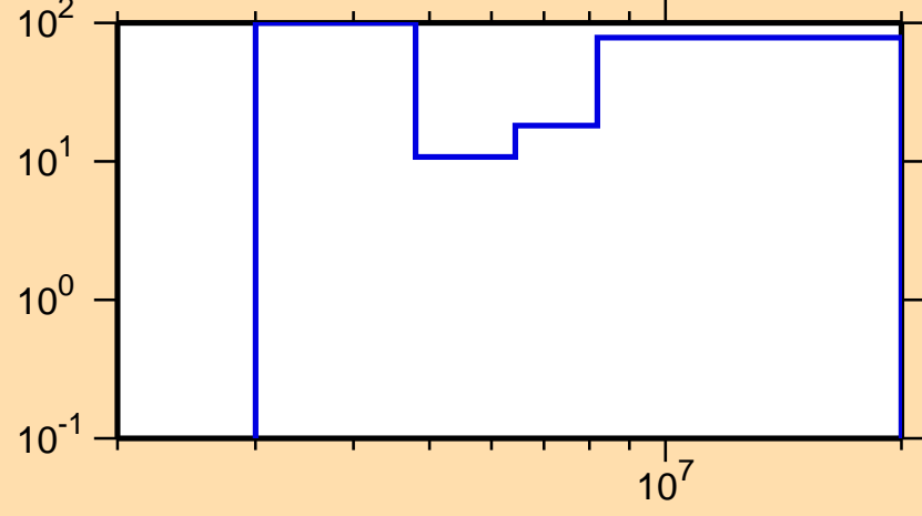
\Delta\sigma/\sigma vs. E for ^{212}\text{Fr}(n,n\text{cont.})
