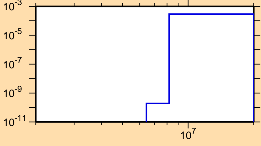
\sigma vs. E for ^{212}\text{Fr}(n,t)
