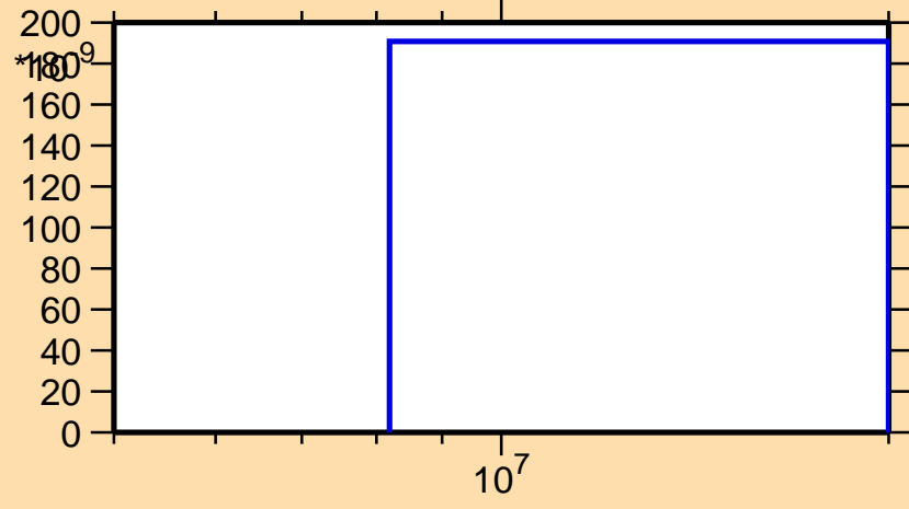
\sigma vs. E for ^{212}\text{Fr}(n,\text{He}3)
