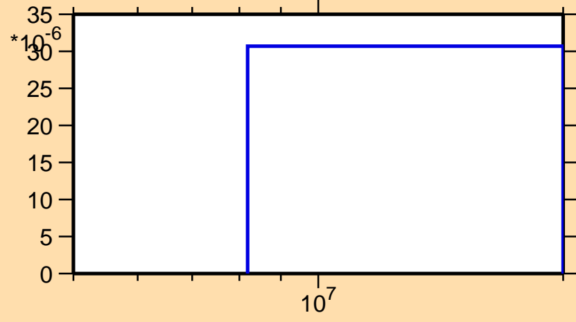
\sigma vs. E for ^{212}\text{Fr}(n,2n\alpha)
