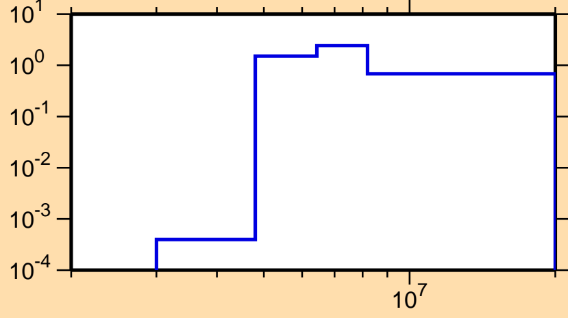
\sigma vs. E for ^{212}\text{Fr}(n,n\text{cont.})
