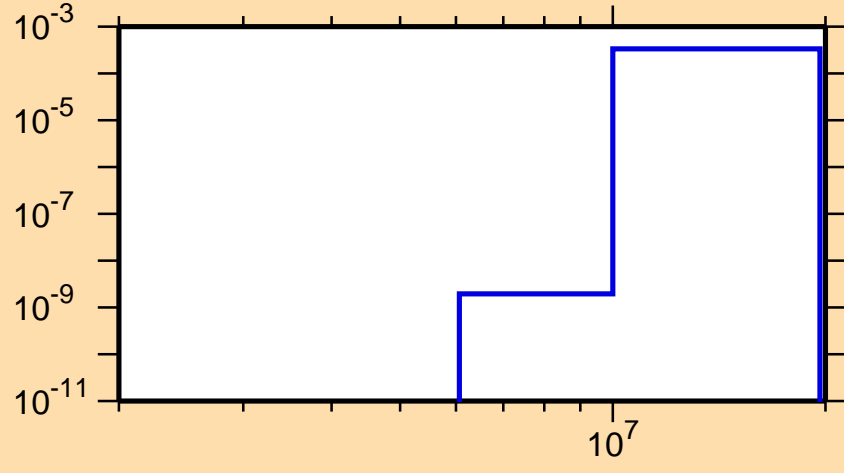
\sigma vs. E for ^{213}\text{Fr}(n,t)
