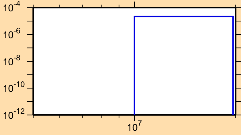
\sigma vs. E for ^{213}\text{Fr}(n,2n\alpha)
