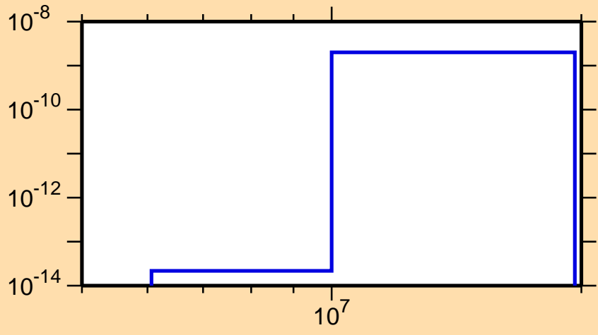
\sigma vs. E for ^{213}\text{Fr}(\text{mt117})
