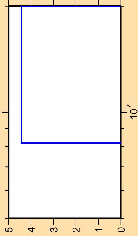
\Delta\sigma/\sigma vs. E for ^{213}\text{Fr}(\text{mt } 34)
