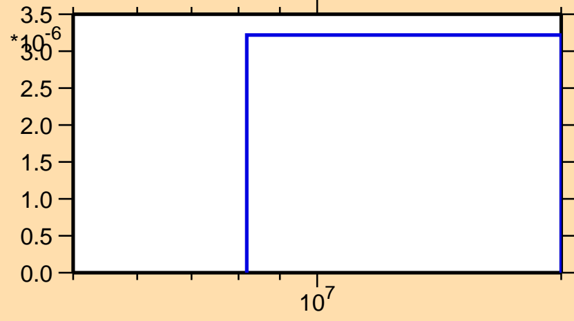
\sigma vs. E for ^{213}\text{Fr}(n,2np)
