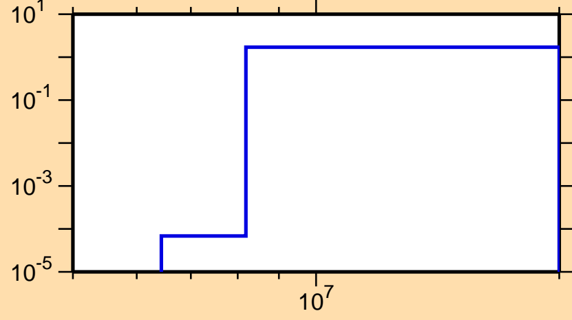
\sigma vs. E for ^{213}\text{Fr}(n,2n)
