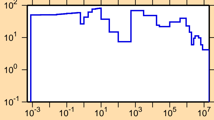
\Delta\sigma/\sigma vs. E for ^{213}\text{Fr}(n,\text{tot.})
