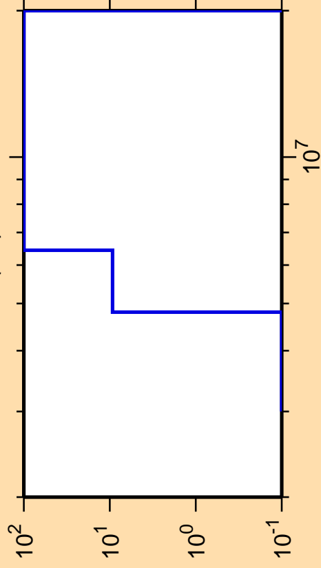
\Delta\sigma/\sigma vs. E for ^{213}\text{Fr}(n,t)
