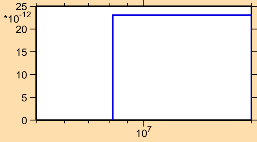
\sigma vs. E for ^{213}\text{Fr}(n,3n\alpha)
