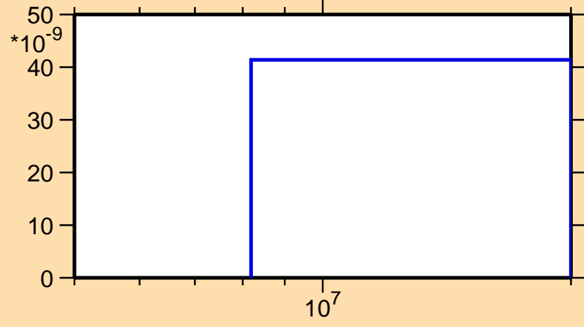
\sigma vs. E for ^{213}\text{Fr}(n,\text{He}3)
