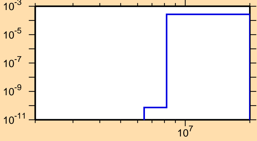
\sigma vs. E for ^{213}\text{Fr}(n,t)
