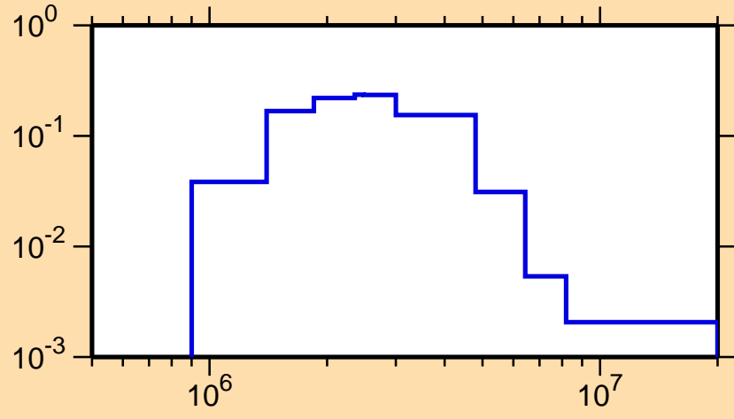
\sigma vs. E for ^{213}\text{Fr}(n,n_2)
