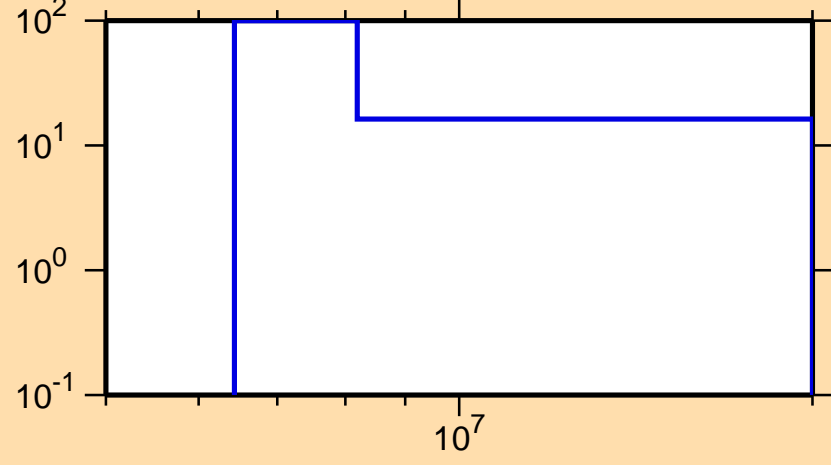
\Delta\sigma/\sigma vs. E for ^{213}\text{Fr}(n,2n)
