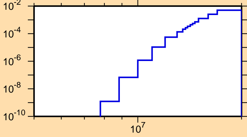
\sigma vs. E for ^{220}\text{Fr}(n,np)
