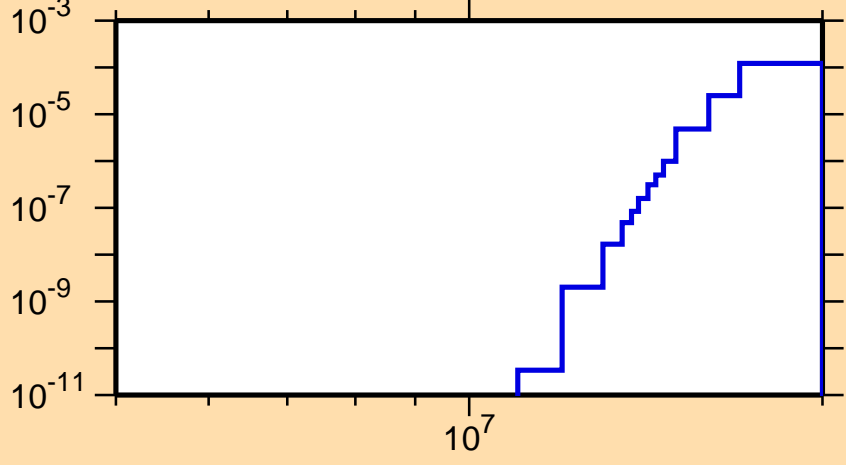
\sigma vs. E for ^{220}\text{Fr}(n,\text{nd})
