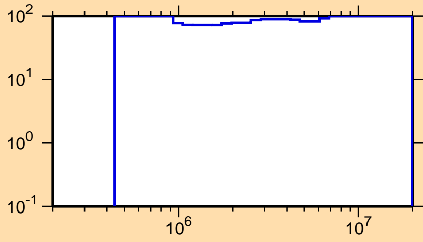
\Delta\sigma/\sigma vs. E for ^{220}\text{Fr}(n,n\text{cont.})
