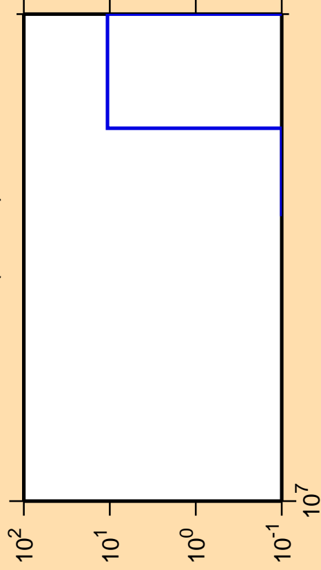
\Delta\sigma/\sigma vs. E for ^{220}\text{Fr}(\text{mt } 42)
