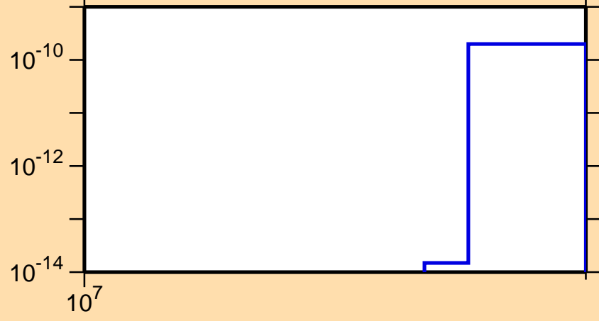
\sigma vs. E for ^{220}\text{Fr}(\text{mt 11})
