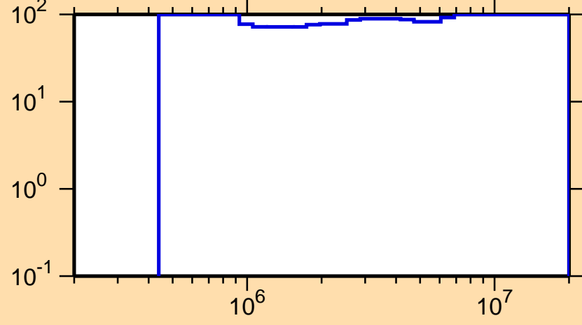
\Delta\sigma/\sigma vs. E for ^{220}\text{Fr}(n,n\text{cont.})
