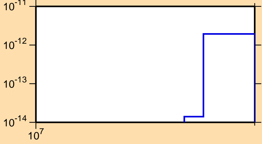
\sigma vs. E for ^{220}\text{Fr} (mt 34)
