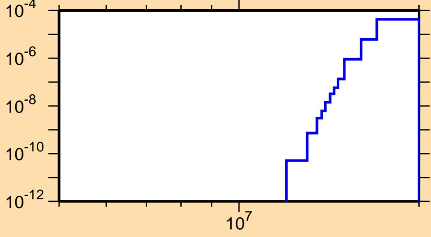
\sigma vs. E for ^{220}\text{Fr}(n,2np)
