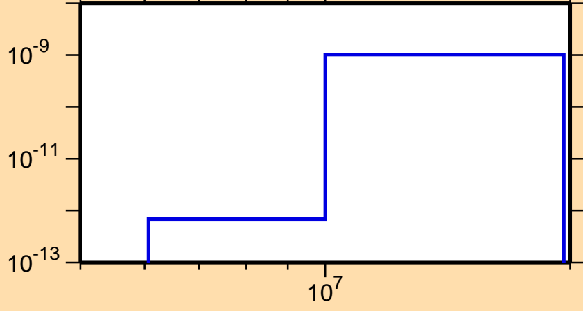
\sigma vs. E for ^{220}\text{Fr}(n,p\alpha)
