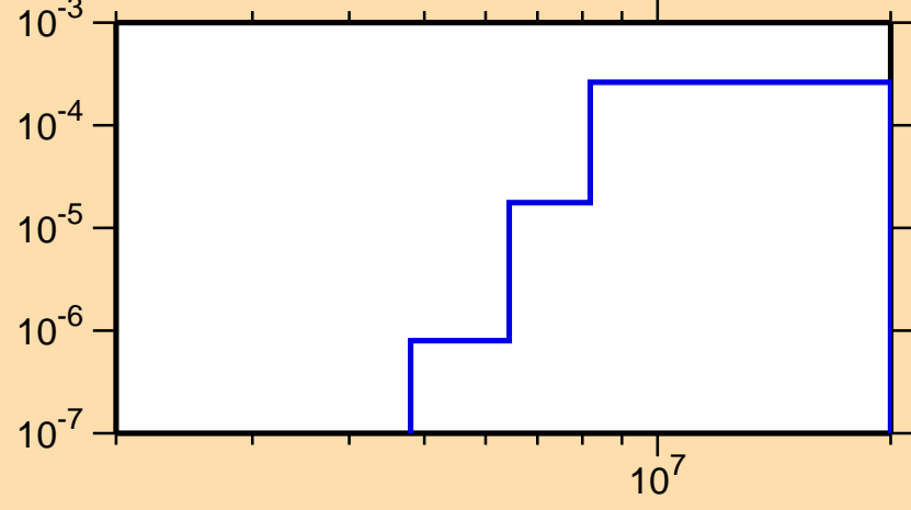
\sigma vs. E for ^{220}\text{Fr}(n,2n\alpha)
