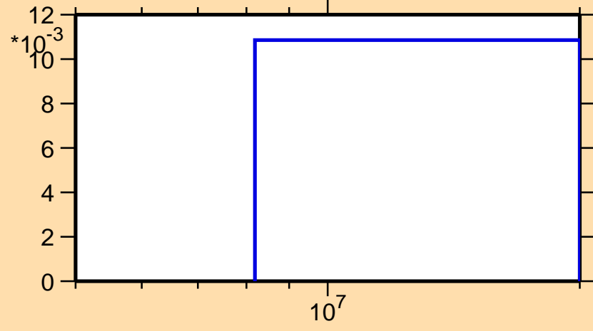
\sigma vs. E for ^{220}\text{Fr}(n,3n\alpha)
