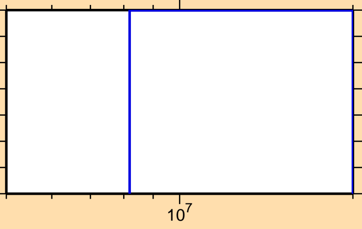
\sigma vs. E for ^{220}\text{Fr}(n,\text{He}3)
