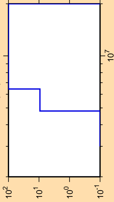
\Delta\sigma/\sigma vs. E for ^{220}\text{Fr}(n,t)
