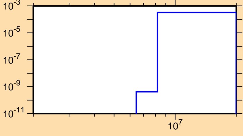
\sigma vs. E for ^{220}\text{Fr}(n,t)
