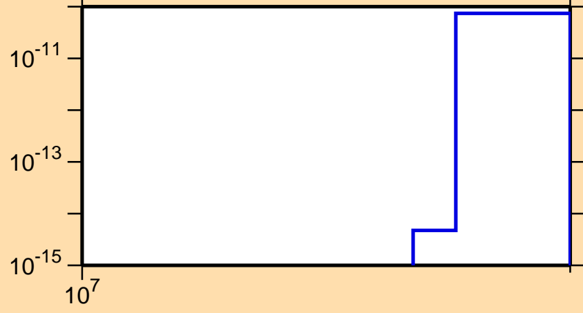
\sigma vs. E for ^{221}\text{Fr}(\text{mt } 11)
