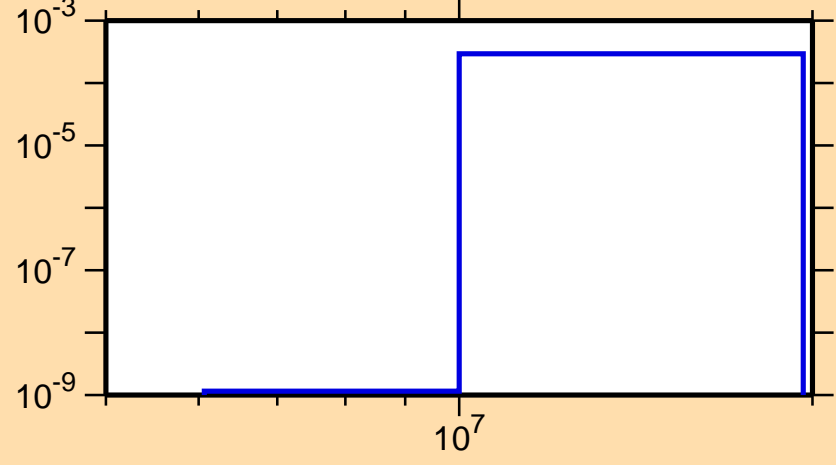
\sigma vs. E for ^{221}\text{Fr}(n,np)
