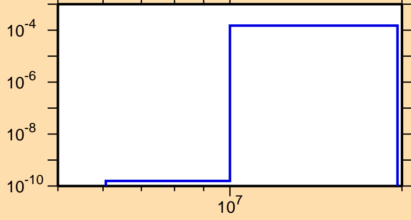
\sigma vs. E for ^{221}\text{Fr}(n,t)
