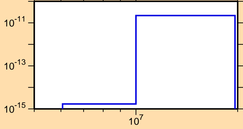
\sigma vs. E for ^{221}\text{Fr}(n,p\alpha)
