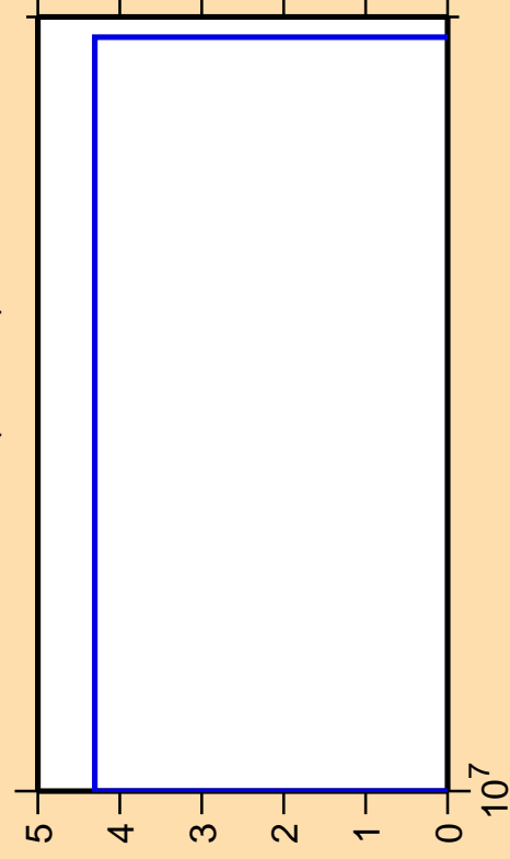
\Delta\sigma/\sigma vs. E for ^{221}\text{Fr}(\text{mt } 45)
