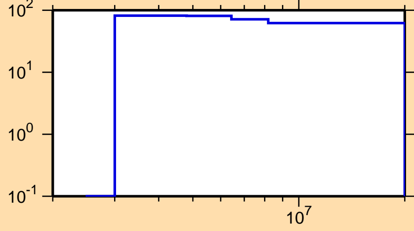
\Delta\sigma/\sigma vs. E for ^{221}\text{Fr}(n,p)
