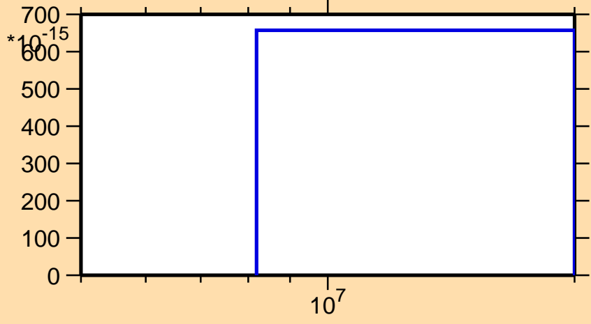
\sigma vs. E for ^{221}\text{Fr}(\text{mt } 45)
