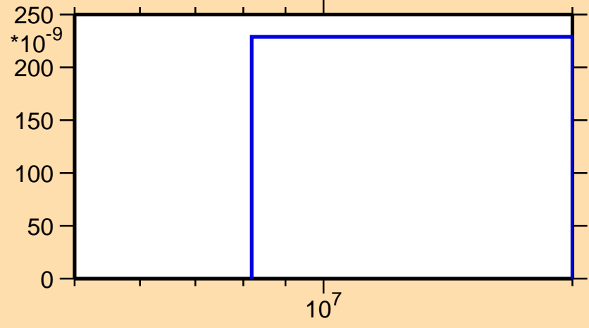
\sigma vs. E for ^{221}\text{Fr}(n,\text{nd})
