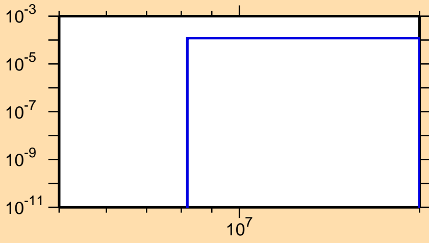
\sigma vs. E for ^{221}\text{Fr}(n,t)
