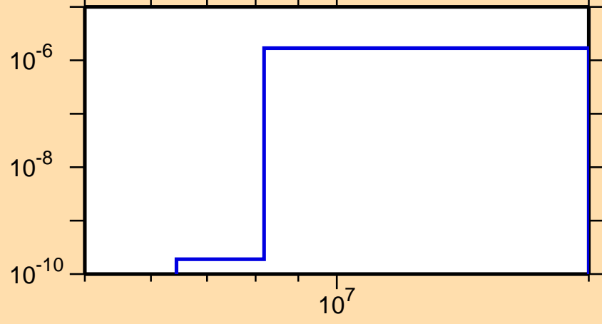
\sigma vs. E for ^{221}\text{Fr}(n,2n\alpha)
