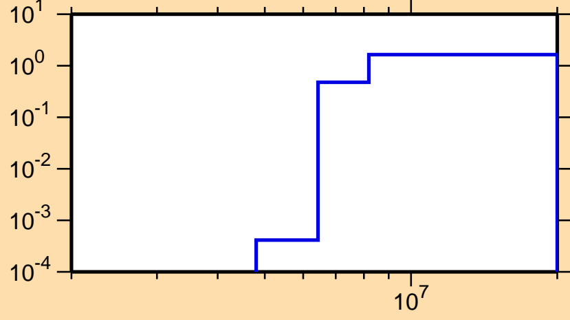
\sigma vs. E for ^{221}\text{Fr}(n,2n)
