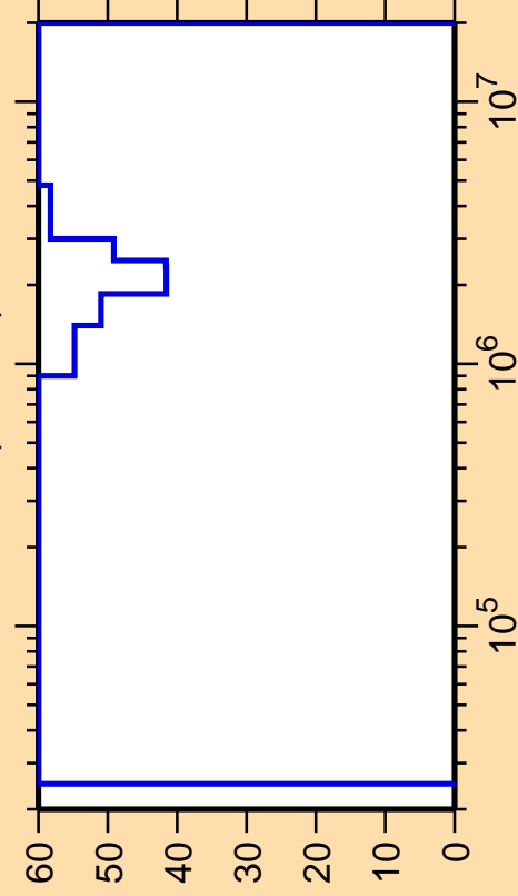
\Delta\sigma/\sigma vs. E for ^{221}\text{Fr}(n,\text{inel.})
