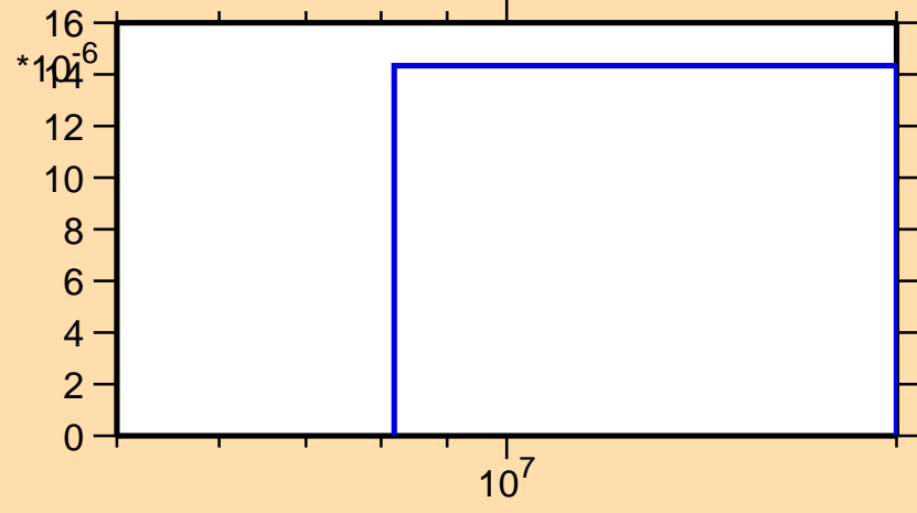
\sigma vs. E for ^{221}\text{Fr}(n,3n\alpha)
