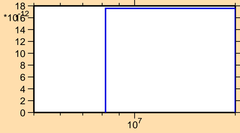
\sigma vs. E for ^{221}\text{Fr}(n,p\alpha)
