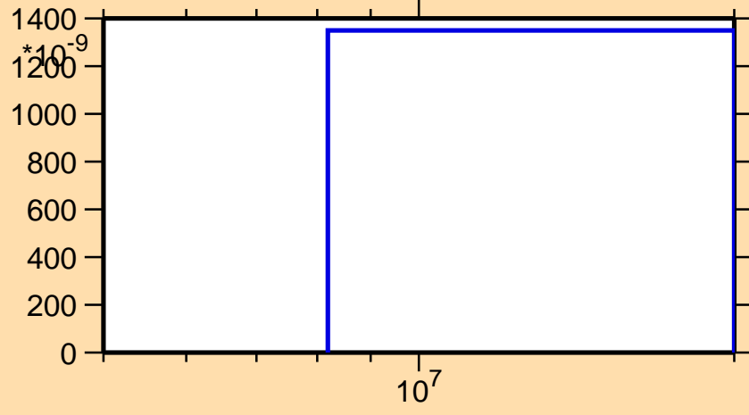
\sigma vs. E for ^{221}\text{Fr}(n,nt)
