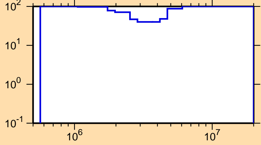
\Delta\sigma/\sigma vs. E for ^{222}\text{Fr}(n,n\text{cont.})
