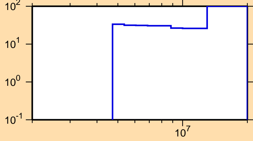
\Delta\sigma/\sigma vs. E for ^{222}\text{Fr}(n,2n)
