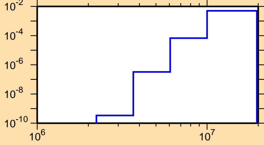
\sigma vs. E for ^{222}\text{Fr}(n,p)
