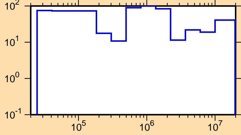
\Delta\sigma/\sigma vs. E for ^{222}\text{Fr}(n,\text{el.})
