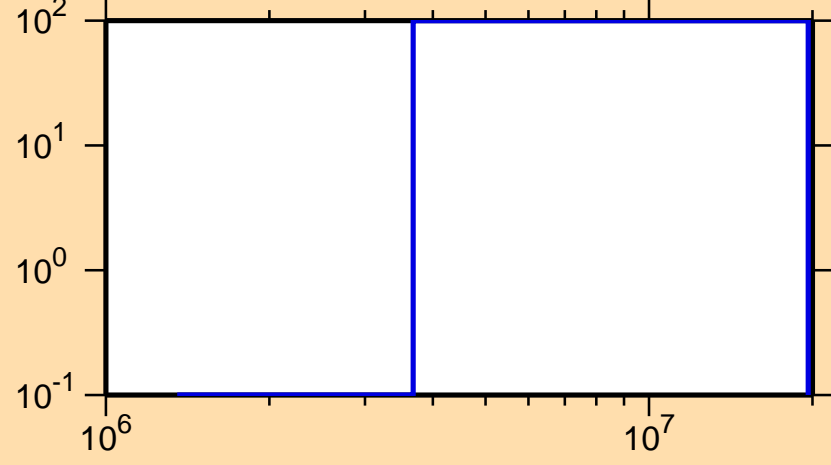
\Delta\sigma/\sigma vs. E for ^{222}\text{Fr}(n,f)
