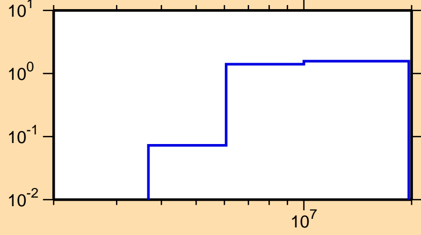
\sigma vs. E for ^{222}\text{Fr}(n,2n)
