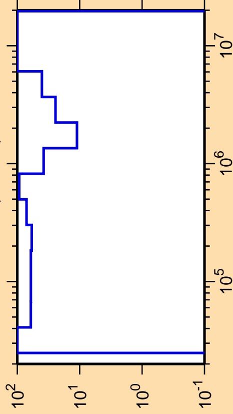
\Delta\sigma/\sigma vs. E for ^{222}\text{Fr}(n,\text{inel.})
