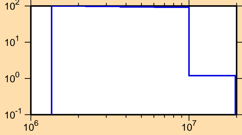
\Delta\sigma/\sigma vs. E for ^{222}\text{Fr}(n,n_1)
