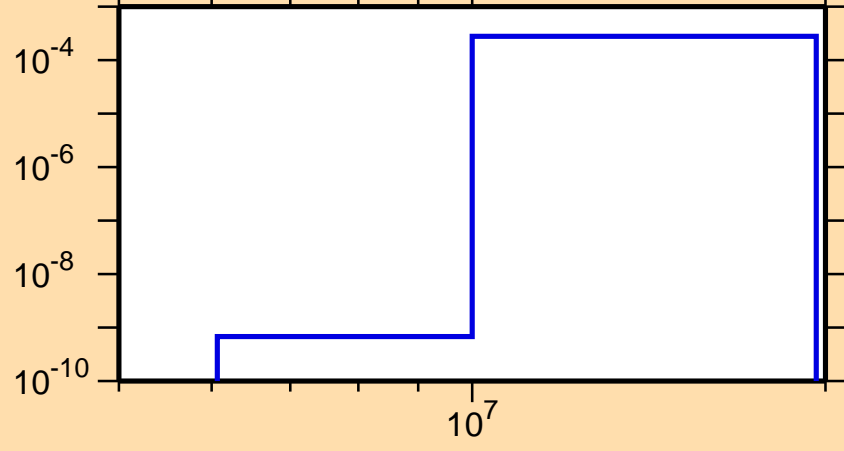
\sigma vs. E for ^{222}\text{Fr}(n,d)
