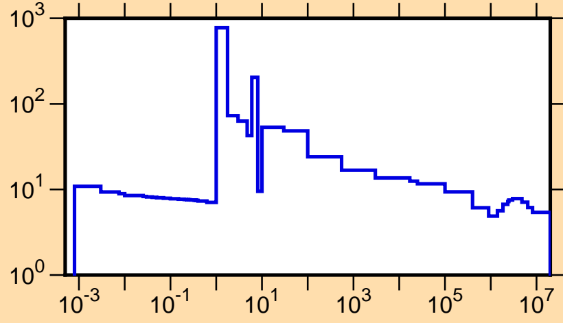
\sigma vs. E for ^{222}\text{Fr}(n,\text{tot.})
