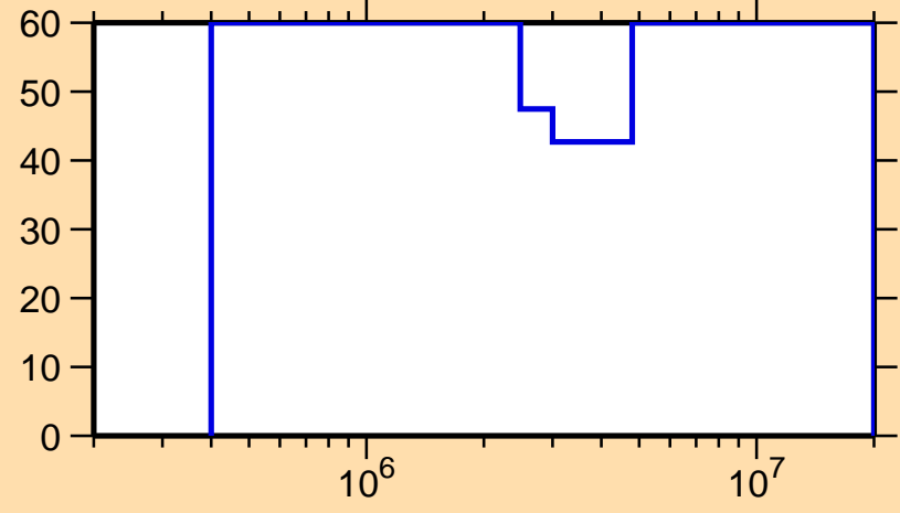
\Delta\sigma/\sigma vs. E for ^{222}\text{Fr}(n,n\text{cont.})
