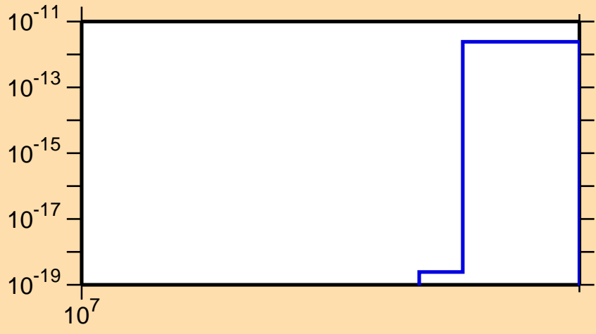
\sigma vs. E for ^{223}\text{Fr}(\text{mt } 42)
