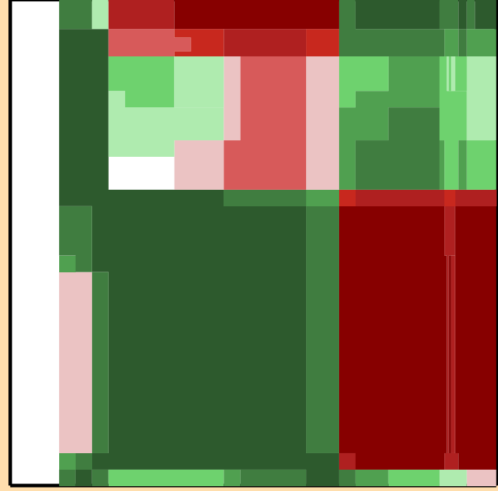
\Delta\sigma/\sigma vs. E for ^{223}\text{Fr}(n,n\text{cont.})
