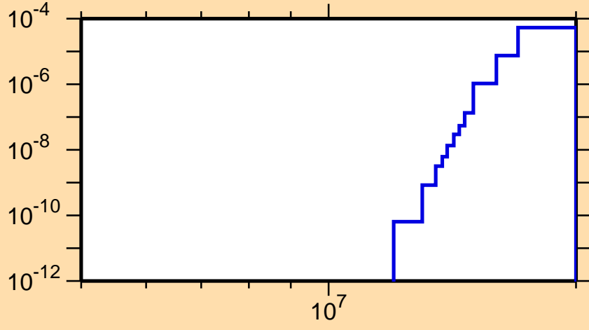
\sigma vs. E for ^{223}\text{Fr}(n,nt)
