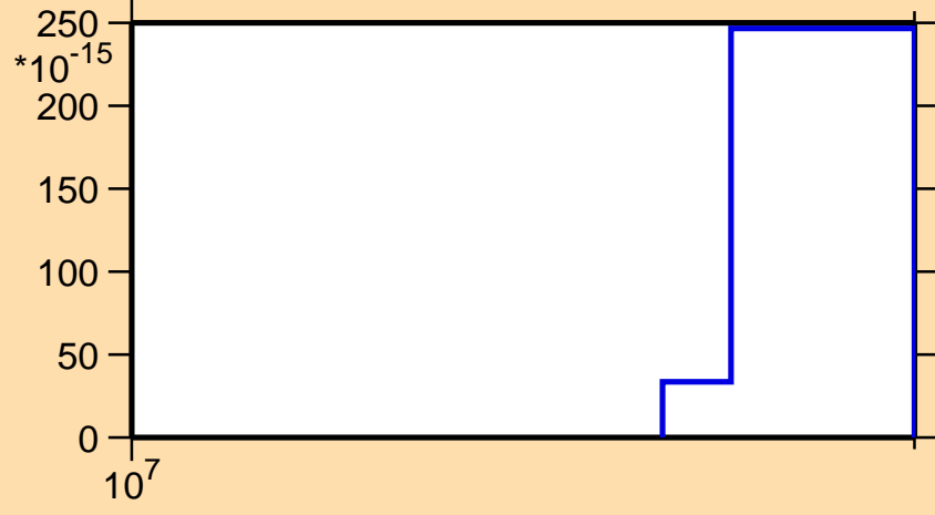
\sigma vs. E for ^{223}\text{Fr}(\text{mt } 45)
