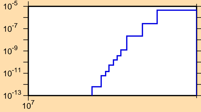
\sigma vs. E for ^{223}\text{Fr}(n,nd)
