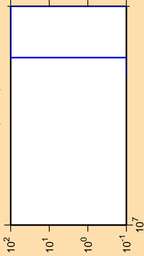
\Delta\sigma/\sigma vs. E for ^{223}\text{Fr} (mt 11)
