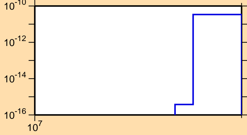
\sigma vs. E for ^{223}\text{Fr} (mt 11)
