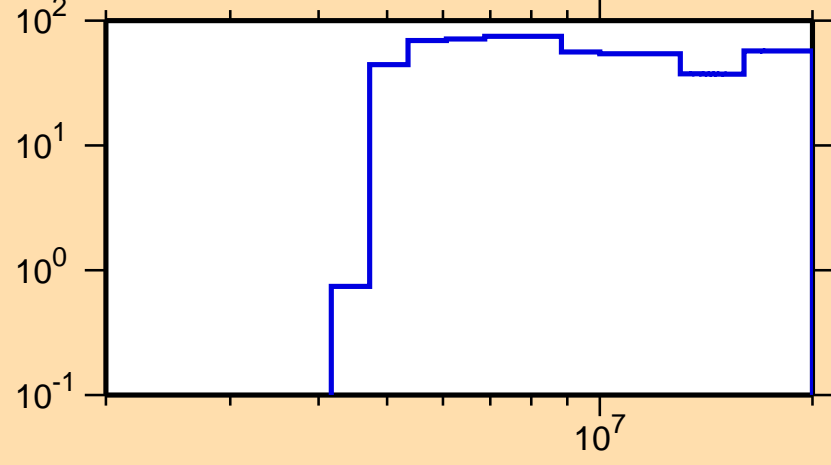
\Delta\sigma/\sigma vs. E for ^{223}\text{Fr}(n,p)
