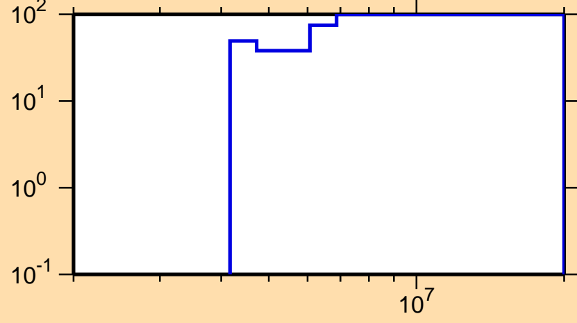
\Delta\sigma/\sigma vs. E for ^{223}\text{Fr}(n,ncont.)
