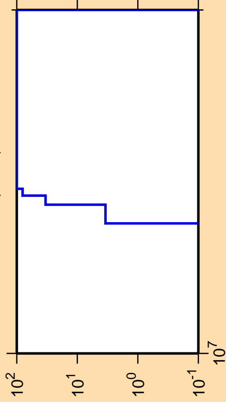
\Delta\sigma/\sigma vs. E for ^{223}\text{Fr}(n,nd)
