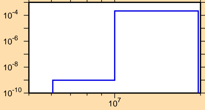
\sigma vs. E for ^{223}\text{Fr}(n,d)
