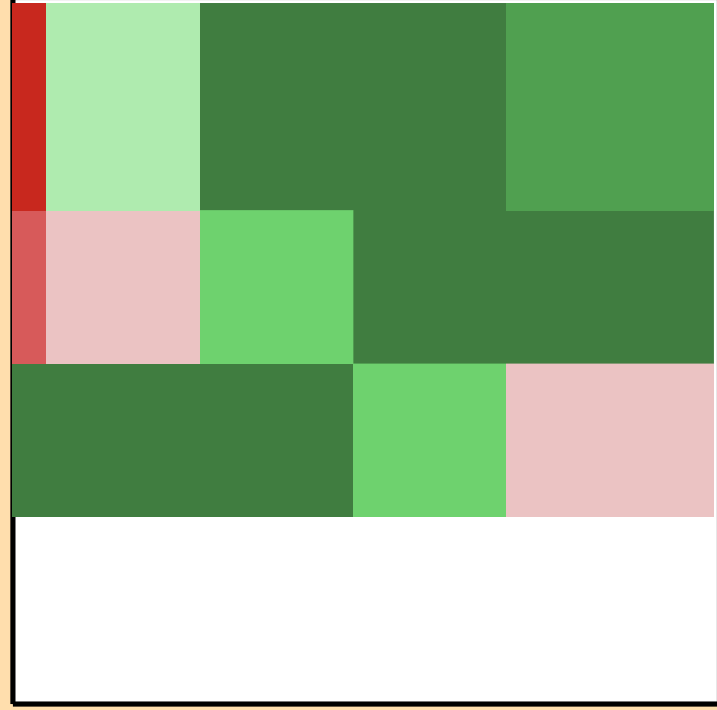
\Delta\sigma/\sigma vs. E for ^{223}\text{Fr}(n,ncont.)
