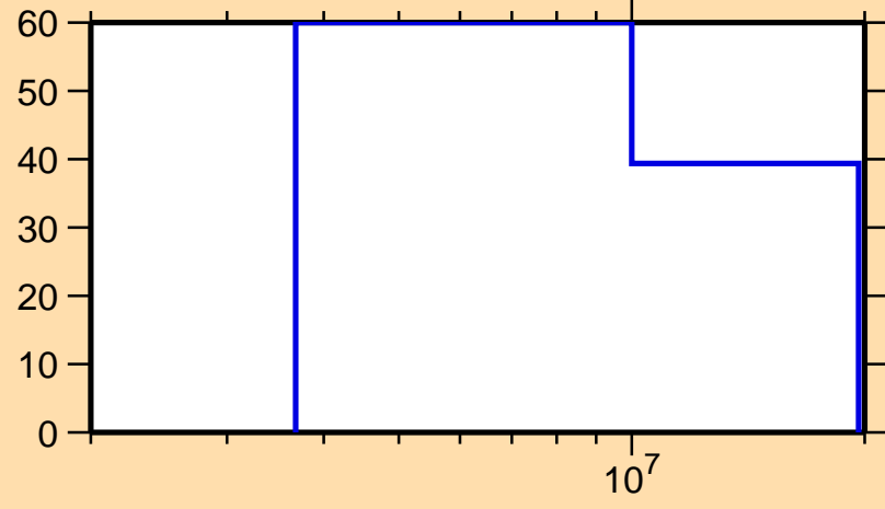
\Delta\sigma/\sigma vs. E for ^{223}\text{Fr}(n,p)
