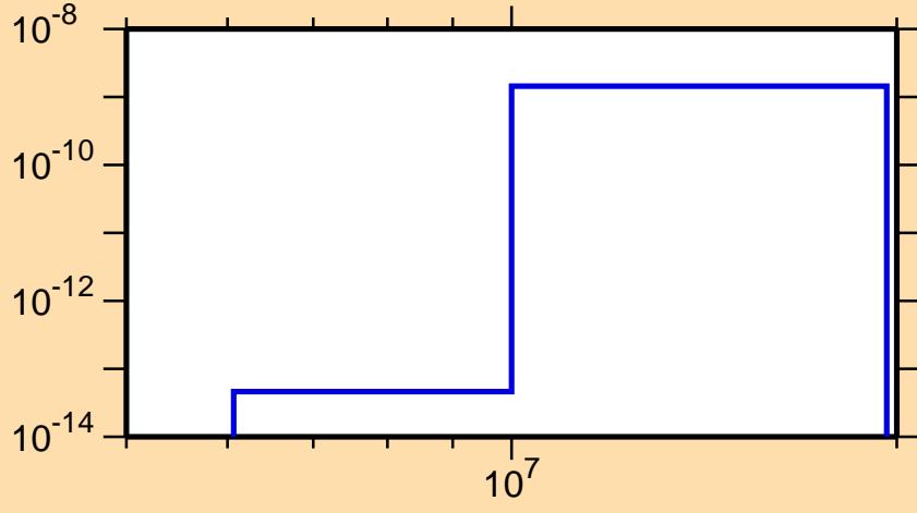
\sigma vs. E for ^{223}\text{Fr}(n,3n\alpha)
