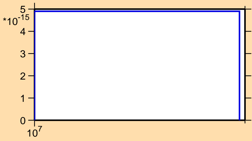
\sigma vs. E for ^{223}\text{Fr}(\text{mt } 45)
