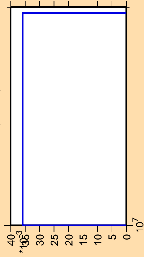
\Delta\sigma/\sigma vs. E for ^{223}\text{Fr}(\text{mt } 45)
