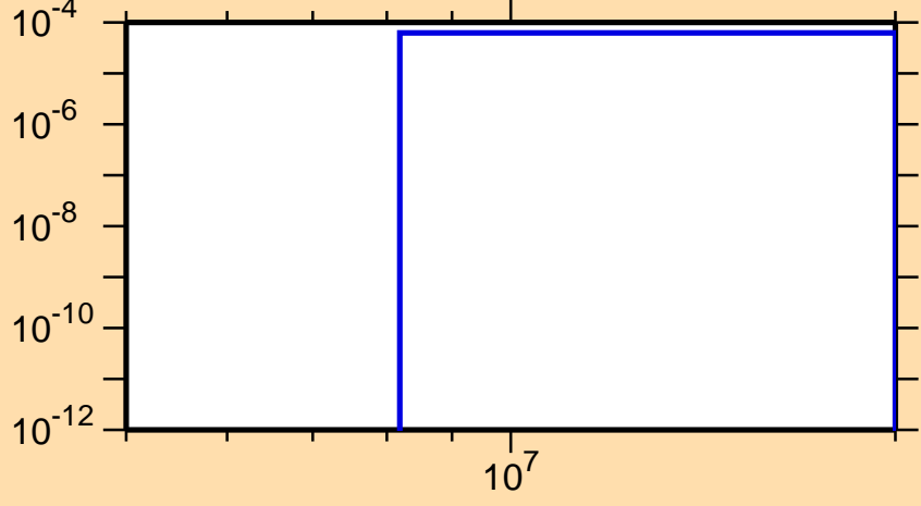
\sigma vs. E for ^{223}\text{Fr}(n,t)
