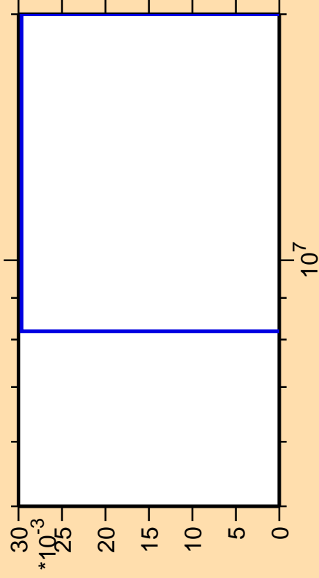
\Delta\sigma/\sigma vs. E for ^{223}\text{Fr} (mt 45)
