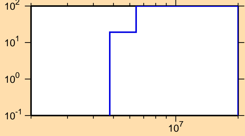
\Delta\sigma/\sigma vs. E for ^{223}\text{Fr}(n,\text{inel.})
