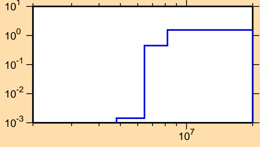
\sigma vs. E for ^{223}\text{Fr}(n,2n)
