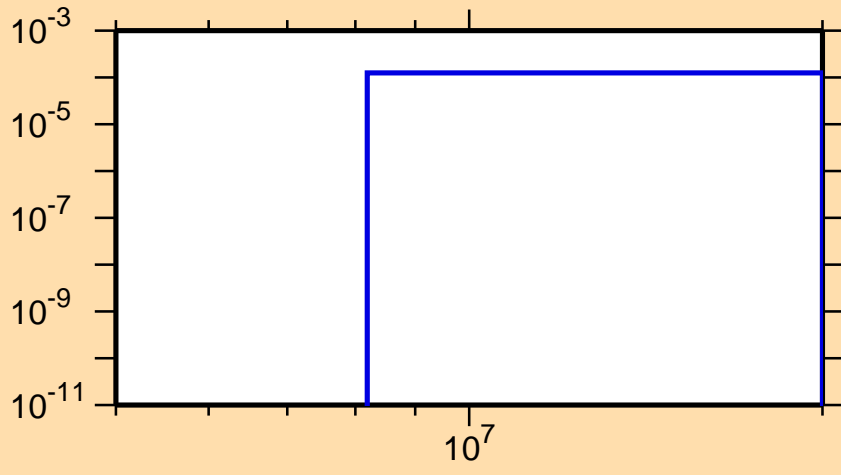
\sigma vs. E for ^{223}\text{Fr}(n,np)
