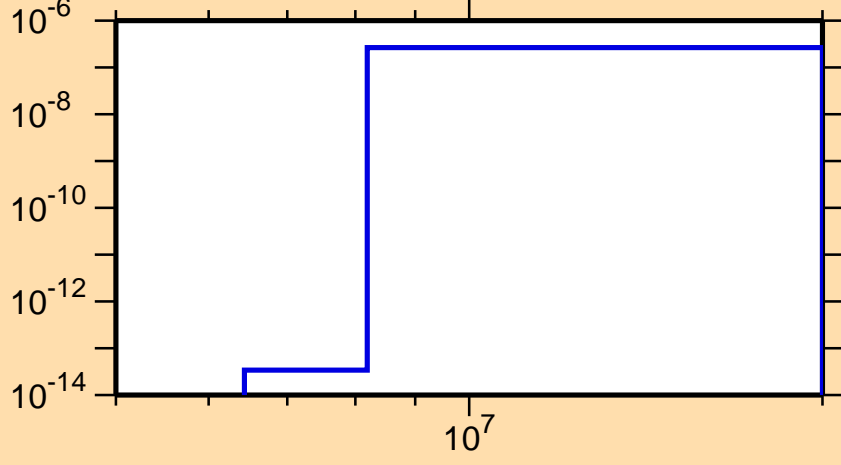
\sigma vs. E for ^{223}\text{Fr}(n,2n\alpha)
