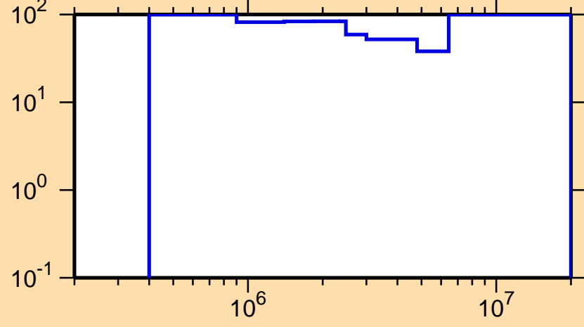
\Delta\sigma/\sigma vs. E for ^{223}\text{Fr}(n,n\text{cont.})
