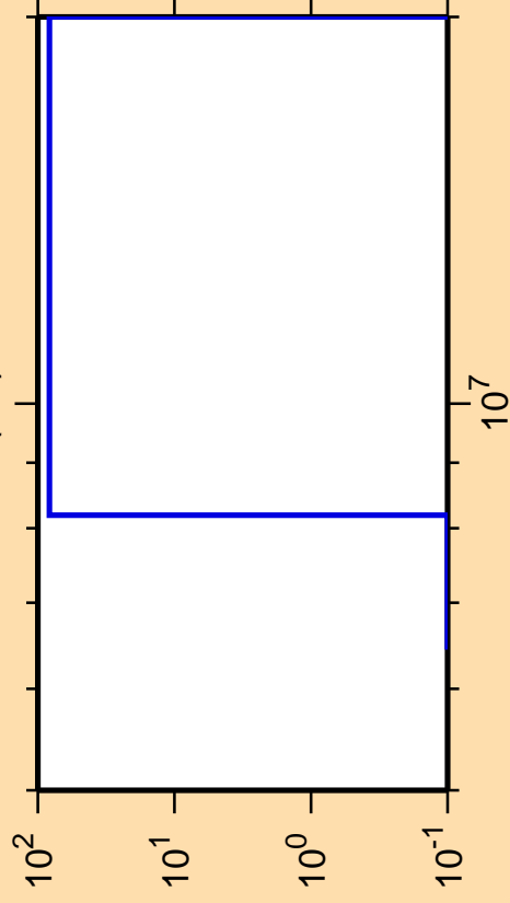
\Delta\sigma/\sigma vs. E for ^{223}\text{Fr}(n,t)
