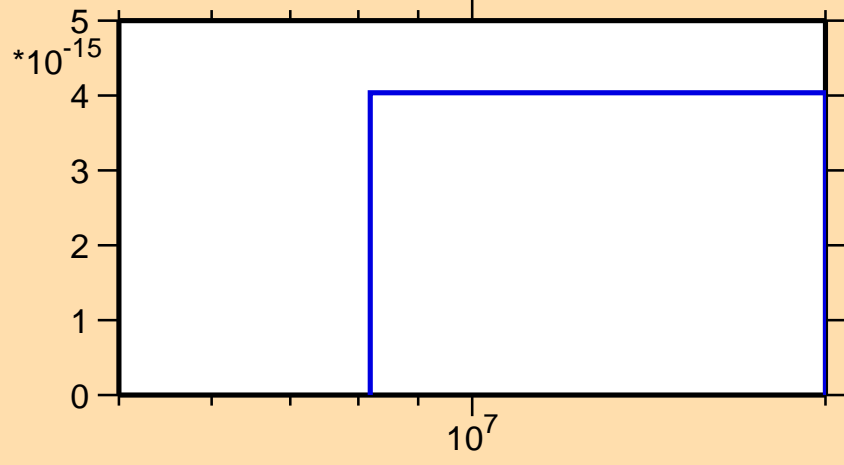
\sigma vs. E for ^{223}\text{Fr} (mt 45)
